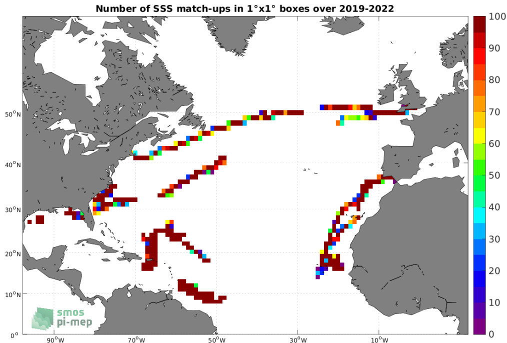
Figure 4: Number of SSS match-ups between Saildrone SSS and the SMAP SSS L3 v5.0 - 8-Day running (JPL) SSS product for the North Atlantic Ocean Pi-MEP region over 1^\circ \times 1^\circ boxes and for the full satellite product period.
