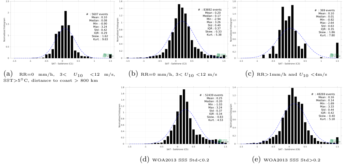
Figure 13: Normalized histogram of \Delta SSS (SMAP SSS L3 v5.0 - 8-Day running (JPL) - Sairdrone) for 5 different subdatasets corresponding to: RR=0 mm/h, 3 < U_{10} < 12 m/s, SST > 5°C, distance to coast > 800 km (a), RR=0 mm/h, 3 < U_{10} < 12 m/s (b), RR > 1mm/h and U_{10} < 4 m/s (c), WOA2013 SSS Std < 0.2 (d), WOA2013 SSS Std > 0.2 (e).
