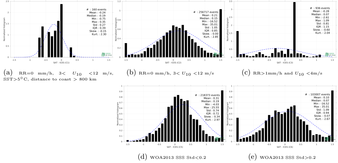
Figure 13: Normalized histogram of \Delta SSS (SMAP SSS L3 v5.0 - 8-Day running (JPL) - ICES) for 5 different subdatasets corresponding to: RR=0 mm/h, 3 < U_{10} < 12 m/s, SST > 5°C, distance to coast > 800 km (a), RR=0 mm/h, 3 < U_{10} < 12 m/s (b), RR > 1mm/h and U_{10} < 4 m/s (c), WOA2013 SSS Std < 0.2 (d), WOA2013 SSS Std > 0.2 (e).
