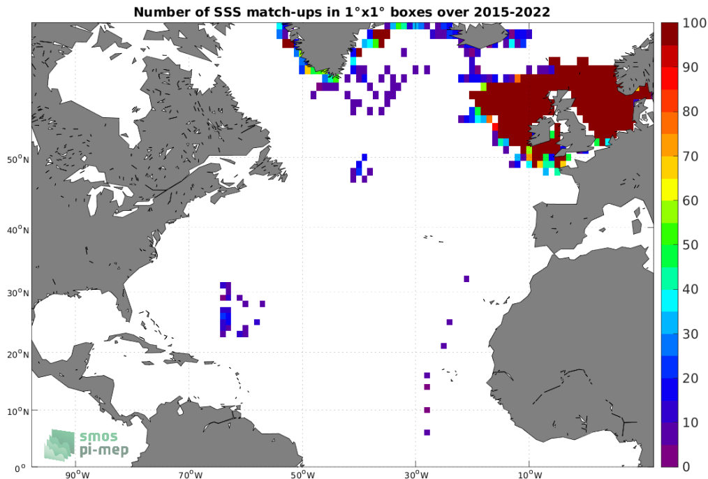
Figure 4: Number of SSS match-ups between ICES SSS and the SMAP SSS L3 v5.0 - 8-Day running (JPL) SSS product for the North Atlantic Ocean Pi-MEP region over 1^\circ \times 1^\circ boxes and for the full satellite product period.
