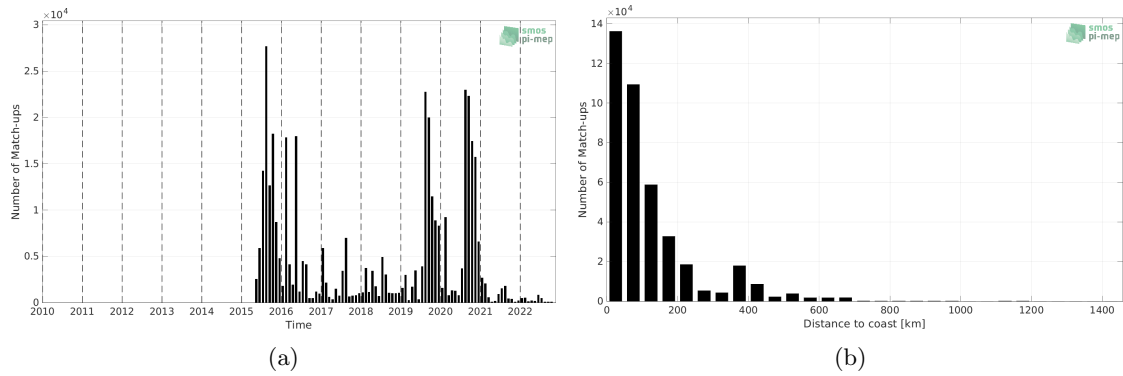
Figure 1: Number of match-ups between ICES and SMAP SSS L3 v5.0 - 8-Day running (JPL) SSS as a function of time (a) and as function of the distance to coast (b) over the North Atlantic Ocean Pi-MEP region and for the full satellite product period.
