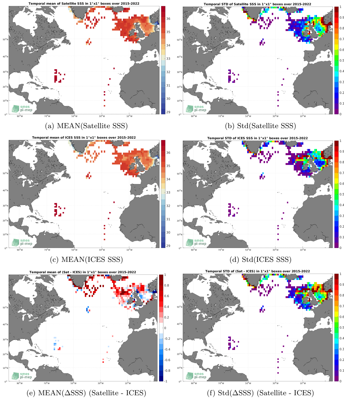
Figure 6: Temporal mean (left) and Std (right) of SSS from SMAP SSS L3 v5.0 - 8-Day running (JPL) (top), ICES (middle), and of \Delta SSS (Satellite - ICES). Only match-up pairs are used to generate these maps.
