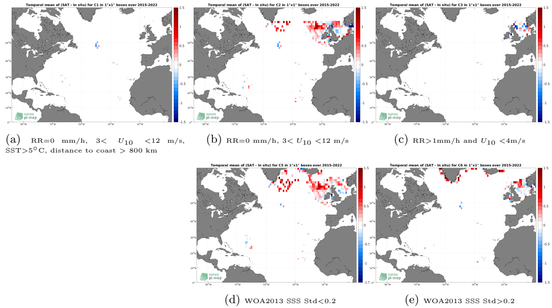
Figure 12: Temporal mean gridded over spatial boxes of size 1^\circ \times 1^\circ of \Delta\text{SSS} (SMAP SSS L3 v5.0 - 8-Day running (JPL) - ICES) for 5 different subdatasets corresponding to:RR=0 mm/h, 3 < U_{10} < 12 m/s, SST >5^\circ\text{C} , distance to coast > 800 km (a), RR=0 mm/h, 3 < U_{10} < 12 m/s (b), RR >1 mm/h and U_{10} < 4 m/s (c), WOA2013 SSS Std <0.2 (d), WOA2013 SSS Std >0.2 (e).
