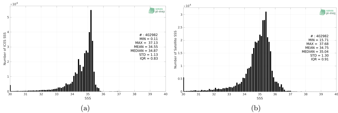
Figure 2: Histograms of SSS from ICES (a) and SMAP SSS L3 v5.0 - 8-Day running (JPL) (b) considering all match-up pairs per bins of 0.1 over the North Atlantic Ocean Pi-MEP region and for the full satellite product period.
