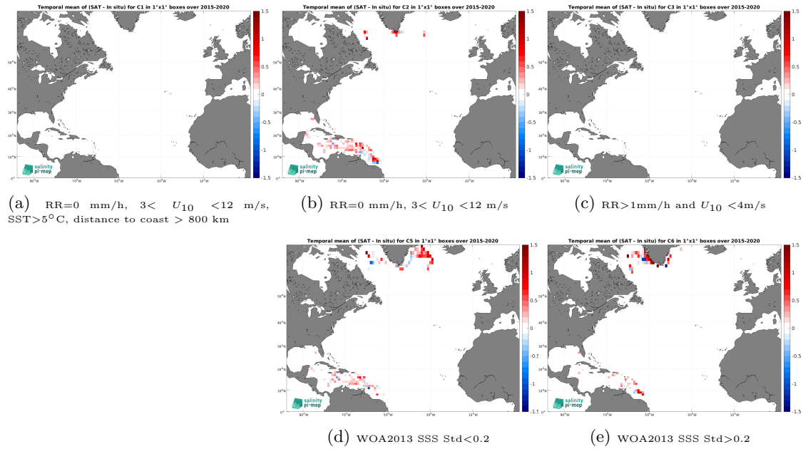
Figure 11: Temporal mean gridded over spatial boxes of size 1^\circ \times 1^\circ of \Delta\text{SSS} (SMAP SSS L3 v5.0 - 8-Day running (JPL) - Surface drifters) for 5 different subdatasets corresponding to:RR=0 mm/h, 3 < U_{10} < 12 m/s, SST >5^\circ\text{C} , distance to coast > 800 km (a), RR=0 mm/h, 3 < U_{10} < 12 m/s (b), RR >1 mm/h and U_{10} < 4 m/s (c), WOA2013 SSS Std <0.2 (d), WOA2013 SSS Std >0.2 (e).
