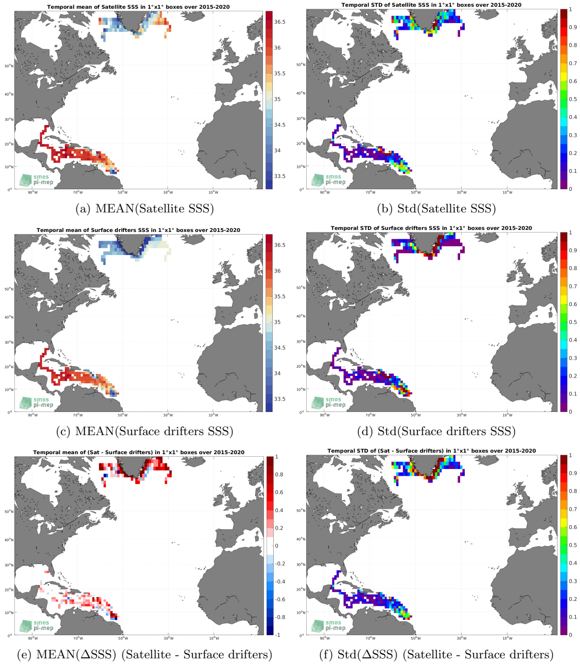
Figure 5: Temporal mean (left) and Std (right) of SSS from SMAP SSS L3 v5.0 - 8-Day running (JPL) (top), Surface drifters (middle), and of \Delta SSS (Satellite - Surface drifters). Only match-up pairs are used to generate these maps.
