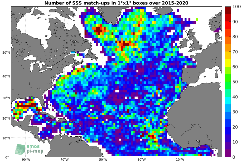
Figure 4: Number of SSS match-ups between Argo SSS and the SMAP SSS L3 v5.0 - 8-Day running (JPL) SSS product for the North Atlantic Ocean Pi-MEP region over 1°x1° boxes and for the full satellite product period.
