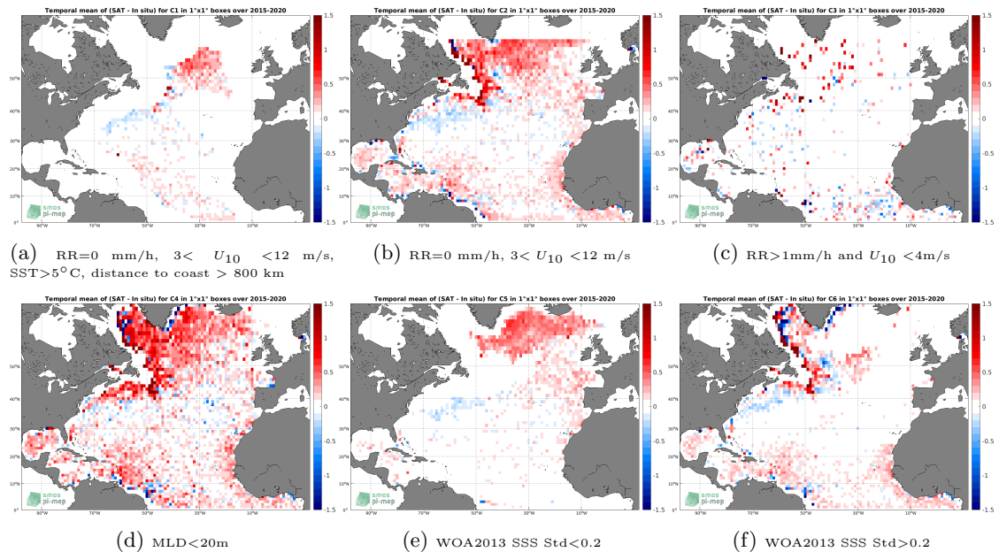
Figure 12: Temporal mean gridded over spatial boxes of size 1°x1° of \Delta SSS (SMAP SSS L3 v5.0 - 8-Day running (JPL) - Argo) for 6 different subdatasets corresponding to:RR=0 mm/h, 3 < U_{10} < 12 m/s, SST>5°C, distance to coast > 800 km (a), RR=0 mm/h, 3 < U_{10} < 12 m/s (b), RR>1mm/h and U_{10} < 4 m/s (c),MLD<20m (d),WOA2013 SSS Std<0.2 (e),WOA2013 SSS Std>0.2 (f).
