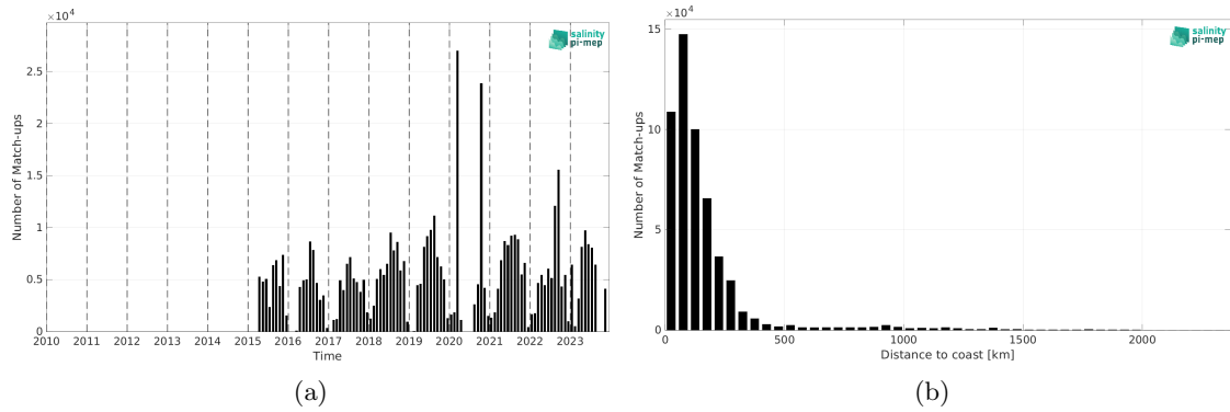
Figure 2: Number of match-ups between TSG (SAMOS) and SMAP SSS L3 v5.0 - Monthly (JPL) SSS as a function of time (a) and as function of the distance to coast (b) over the North Atlantic Ocean Pi-MEP region and for the full satellite product period.
