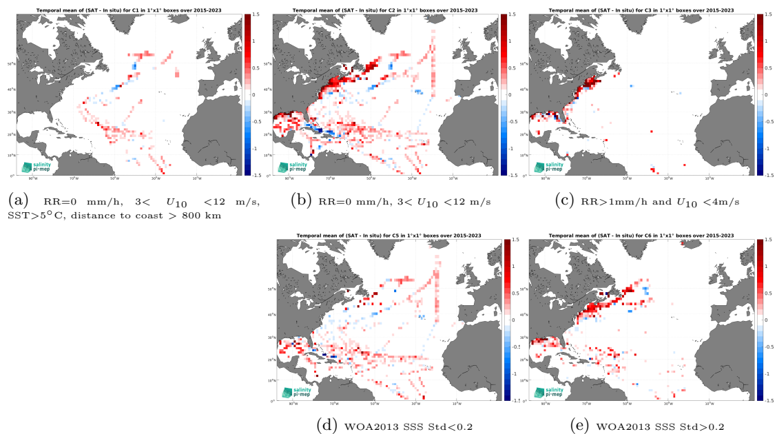
Figure 14: Temporal mean gridded over spatial boxes of size 1^\circ \times 1^\circ of \Delta\text{SSS} (SMAP SSS L3 v5.0 - Monthly (JPL) - TSG (SAMOS)) for 5 different subdatasets corresponding to: RR=0 mm/h, 3 < U_{10} < 12 m/s, SST > 5°C, distance to coast > 800 km (a), RR=0 mm/h, 3 < U_{10} < 12 m/s (b), RR > 1mm/h and U_{10} < 4 m/s (c), WOA2013 SSS Std < 0.2 (d), WOA2013 SSS Std > 0.2 (e).
