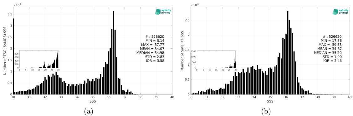
Figure 3: Histograms of SSS from TSG (SAMOS) (a) and SMAP SSS L3 v5.0 - Monthly (JPL) (b) considering all match-up pairs per bins of 0.1 over the North Atlantic Ocean Pi-MEP region and for the full satellite product period.
