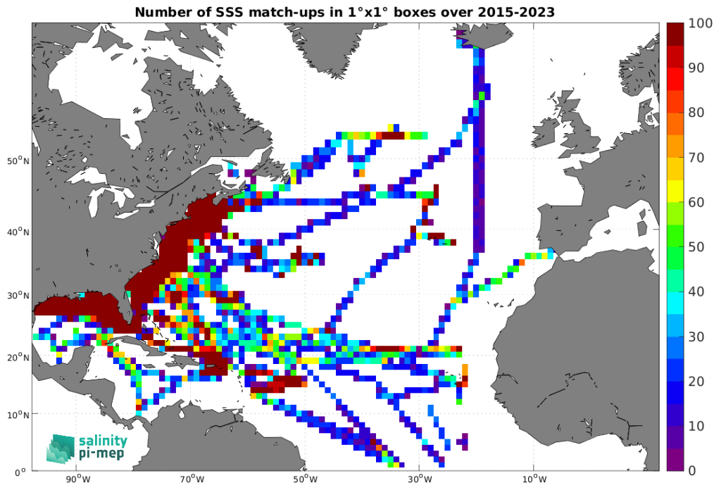
Figure 5: Number of SSS match-ups between TSG (SAMOS) SSS and the SMAP SSS L3 v5.0 - Monthly (JPL) SSS product for the North Atlantic Ocean Pi-MEP region over 1^\circ \times 1^\circ boxes and for the full satellite product period.
