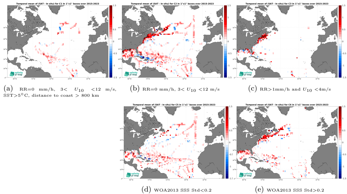
Figure 12: Temporal mean gridded over spatial boxes of size 1^\circ \times 1^\circ of \Delta\text{SSS} (SMAP SSS L3 v5.0 - Monthly (JPL) - TSG (SAMOS)) for 5 different subdatasets corresponding to:RR=0 mm/h, 3 < U_{10} < 12 m/s, SST >5^\circ\text{C} , distance to coast > 800 km (a), RR=0 mm/h, 3 < U_{10} < 12 m/s (b), RR >1 mm/h and U_{10} < 4 m/s (c), WOA2013 SSS Std <0.2 (d), WOA2013 SSS Std >0.2 (e).
