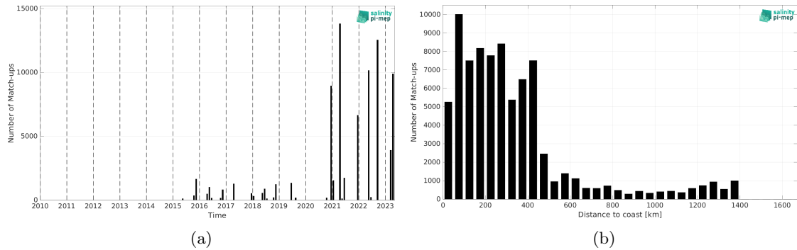
Figure 2: Number of match-ups between TSG (Polarstern) and SMAP SSS L3 v5.0 - Monthly (JPL) SSS as a function of time (a) and as function of the distance to coast (b) over the North Atlantic Ocean Pi-MEP region and for the full satellite product period.
