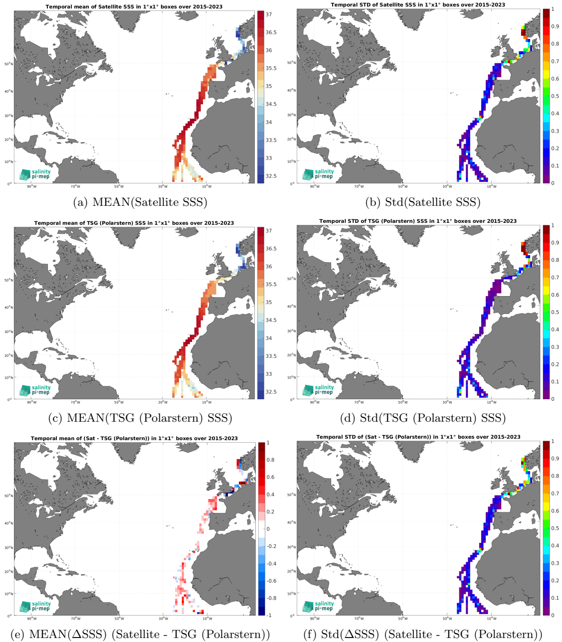
Figure 7: Temporal mean (left) and Std (right) of SSS from SMAP SSS L3 v5.0 - Monthly (JPL) (top), TSG (Polarstern) (middle), and of \Delta SSS (Satellite - TSG (Polarstern)). Only match-up pairs are used to generate these maps.
