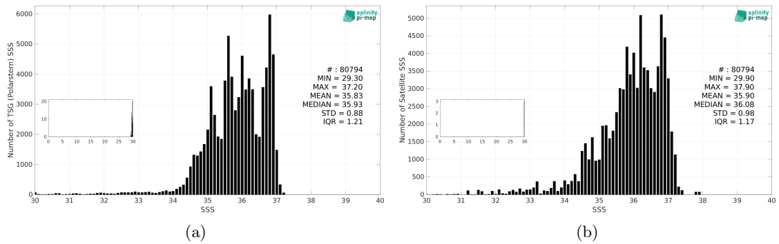
Figure 3: Histograms of SSS from TSG (Polarstern) (a) and SMAP SSS L3 v5.0 - Monthly (JPL) (b) considering all match-up pairs per bins of 0.1 over the North Atlantic Ocean Pi-MEP region and for the full satellite product period.
