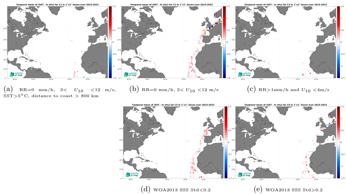
Figure 14: Temporal mean gridded over spatial boxes of size 1^\circ \times 1^\circ of \Delta\text{SSS} (SMAP SSS L3 v5.0 - Monthly (JPL) - TSG (Polarstern)) for 5 different subdatasets corresponding to:RR=0 mm/h, 3 < U_{10} < 12 m/s, SST >5^\circ\text{C} , distance to coast > 800 km (a), RR=0 mm/h, 3 < U_{10} < 12 m/s (b), RR >1 mm/h and U_{10} < 4 m/s (c), WOA2013 SSS Std <0.2 (d), WOA2013 SSS Std >0.2 (e).
