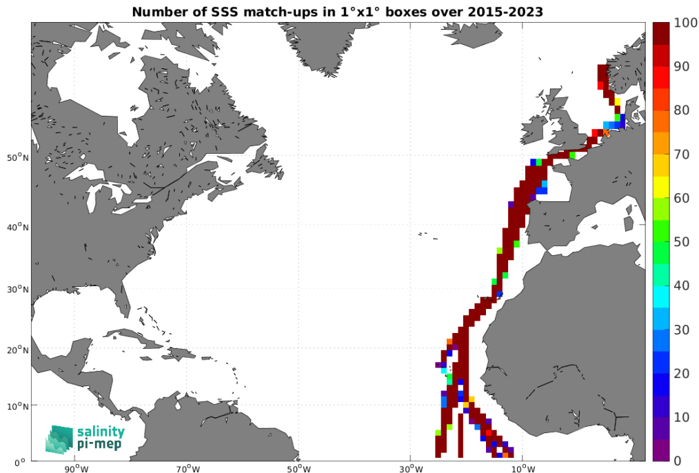
Figure 5: Number of SSS match-ups between TSG (Polarstern) SSS and the SMAP SSS L3 v5.0 - Monthly (JPL) SSS product for the North Atlantic Ocean Pi-MEP region over 1^\circ \times 1^\circ boxes and for the full satellite product period.
