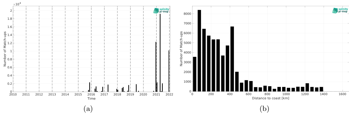
Figure 1: Number of match-ups between TSG (Polarstern) and SMAP SSS L3 v5.0 - Monthly (JPL) SSS as a function of time (a) and as function of the distance to coast (b) over the North Atlantic Ocean Pi-MEP region and for the full satellite product period.
