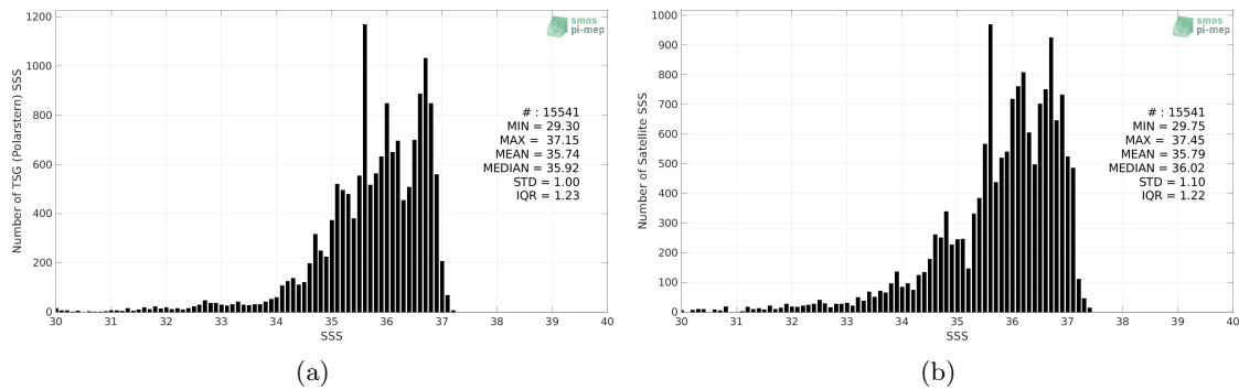
Figure 2: Histograms of SSS from TSG (Polarstern) (a) and SMAP SSS L3 v5.0 - Monthly (JPL) (b) considering all match-up pairs per bins of 0.1 over the North Atlantic Ocean Pi-MEP region and for the full satellite product period.
