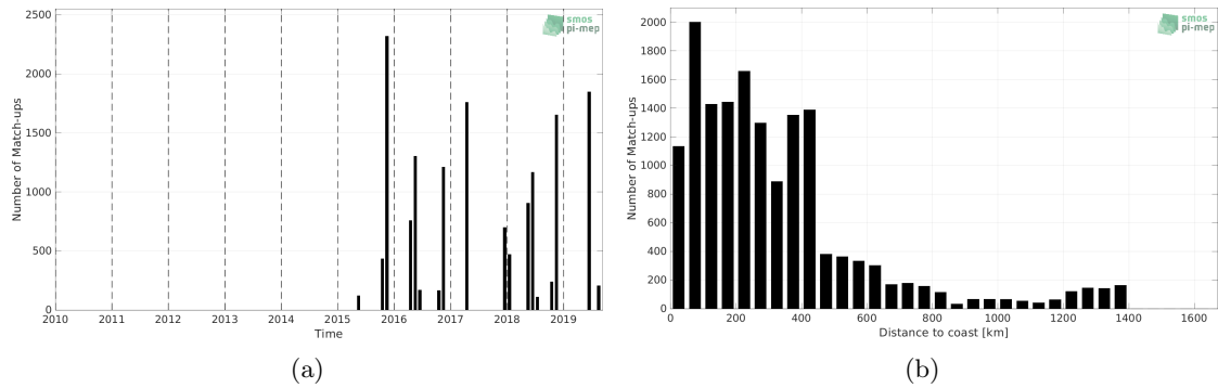
Figure 1: Number of match-ups between TSG (Polarstern) and SMAP SSS L3 v5.0 - Monthly (JPL) SSS as a function of time (a) and as function of the distance to coast (b) over the North Atlantic Ocean Pi-MEP region and for the full satellite product period.
