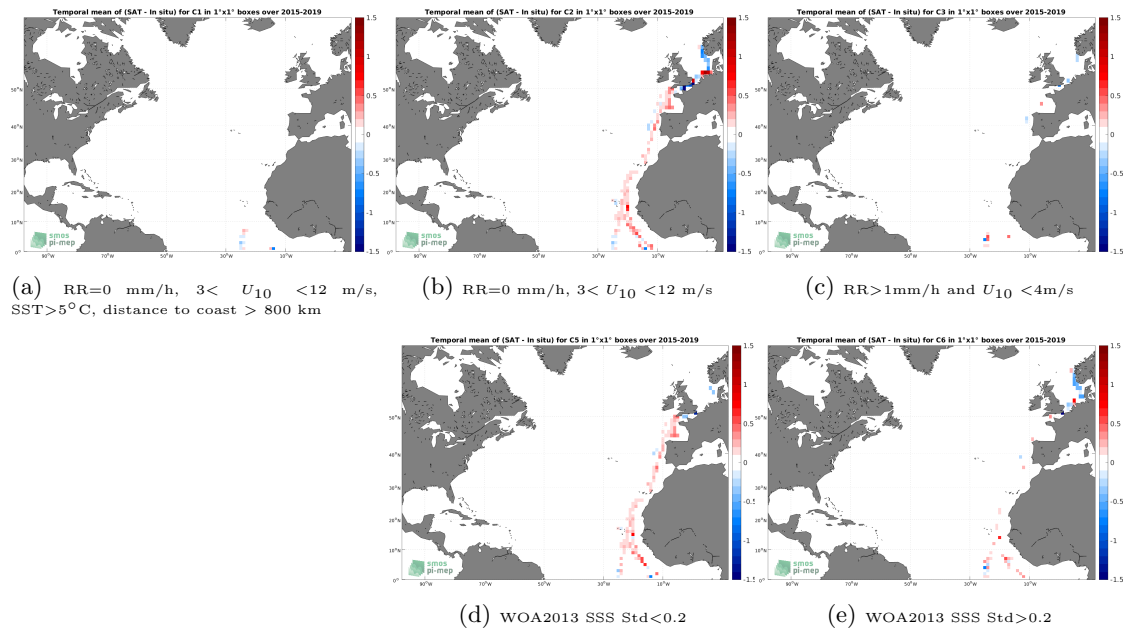
Figure 12: Temporal mean gridded over spatial boxes of size 1^\circ \times 1^\circ of \Delta\text{SSS} (SMAP SSS L3 v5.0 - Monthly (JPL) - TSG (Polarstern)) for 5 different subdatasets corresponding to:RR=0 mm/h, 3 < U_{10} < 12 m/s, SST >5^\circ\text{C} , distance to coast > 800 km (a), RR=0 mm/h, 3 < U_{10} < 12 m/s (b), RR >1 mm/h and U_{10} < 4 m/s (c), WOA2013 SSS Std <0.2 (d), WOA2013 SSS Std >0.2 (e).
