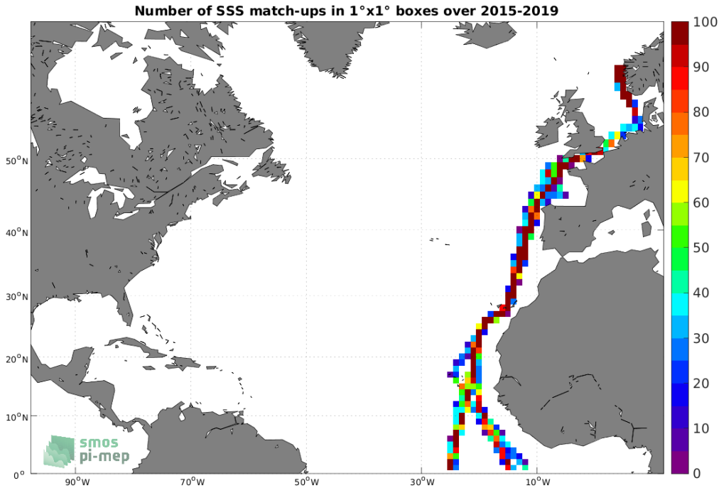
Figure 4: Number of SSS match-ups between TSG (Polarstern) SSS and the SMAP SSS L3 v5.0 - Monthly (JPL) SSS product for the North Atlantic Ocean Pi-MEP region over 1°x1° boxes and for the full satellite product period.
