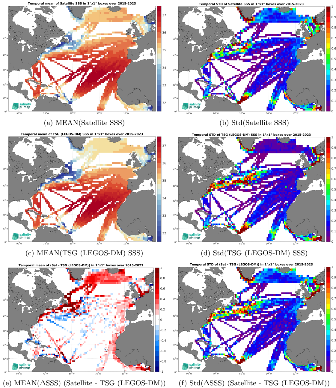
Figure 7: Temporal mean (left) and Std (right) of SSS from SMAP SSS L3 v5.0 - Monthly (JPL) (top), TSG (LEGOS-DM) (middle), and of \Delta SSS (Satellite - TSG (LEGOS-DM)). Only match-up pairs are used to generate these maps.
