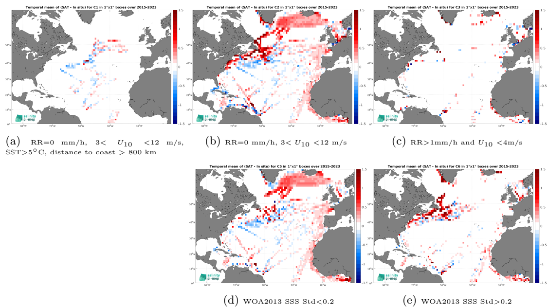
Figure 14: Temporal mean gridded over spatial boxes of size 1^\circ \times 1^\circ of \Delta\text{SSS} (SMAP SSS L3 v5.0 - Monthly (JPL) - TSG (LEGOS-DM)) for 5 different subdatasets corresponding to:RR=0 mm/h, 3 < U_{10} < 12 m/s, SST >5^\circ\text{C} , distance to coast > 800 km (a), RR=0 mm/h, 3 < U_{10} < 12 m/s (b), RR >1 mm/h and U_{10} < 4 m/s (c), WOA2013 SSS Std <0.2 (d), WOA2013 SSS Std >0.2 (e).
