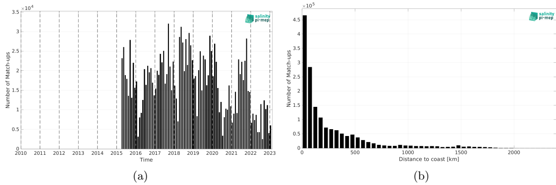
Figure 2: Number of match-ups between TSG (LEGOS-DM) and SMAP SSS L3 v5.0 - Monthly (JPL) SSS as a function of time (a) and as function of the distance to coast (b) over the North Atlantic Ocean Pi-MEP region and for the full satellite product period.
