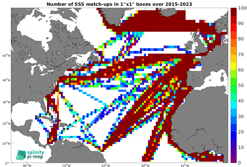
Figure 5: Number of SSS match-ups between TSG (LEGOS-DM) SSS and the SMAP SSS L3 v5.0 - Monthly (JPL) SSS product for the North Atlantic Ocean Pi-MEP region over 1^\circ \times 1^\circ boxes and for the full satellite product period.
