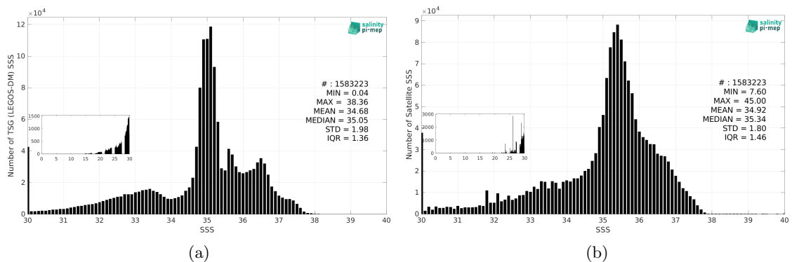
Figure 3: Histograms of SSS from TSG (LEGOS-DM) (a) and SMAP SSS L3 v5.0 - Monthly (JPL) (b) considering all match-up pairs per bins of 0.1 over the North Atlantic Ocean Pi-MEP region and for the full satellite product period.
