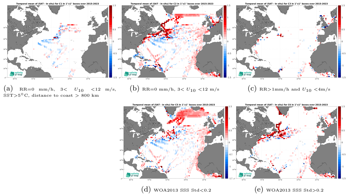
Figure 12: Temporal mean gridded over spatial boxes of size 1^\circ \times 1^\circ of \Delta\text{SSS} (SMAP SSS L3 v5.0 - Monthly (JPL) - TSG (LEGOS-DM)) for 5 different subdatasets corresponding to:RR=0 mm/h, 3 < U_{10} < 12 m/s, SST >5^\circ\text{C} , distance to coast > 800 km (a), RR=0 mm/h, 3 < U_{10} < 12 m/s (b), RR >1 mm/h and U_{10} < 4 m/s (c), WOA2013 SSS Std <0.2 (d), WOA2013 SSS Std >0.2 (e).
