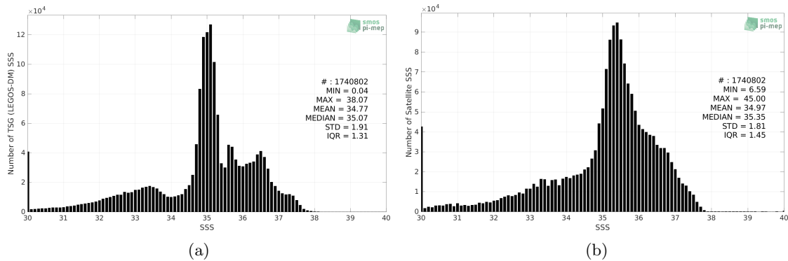
Figure 2: Histograms of SSS from TSG (LEGOS-DM) (a) and SMAP SSS L3 v5.0 - Monthly (JPL) (b) considering all match-up pairs per bins of 0.1 over the North Atlantic Ocean Pi-MEP region and for the full satellite product period.
