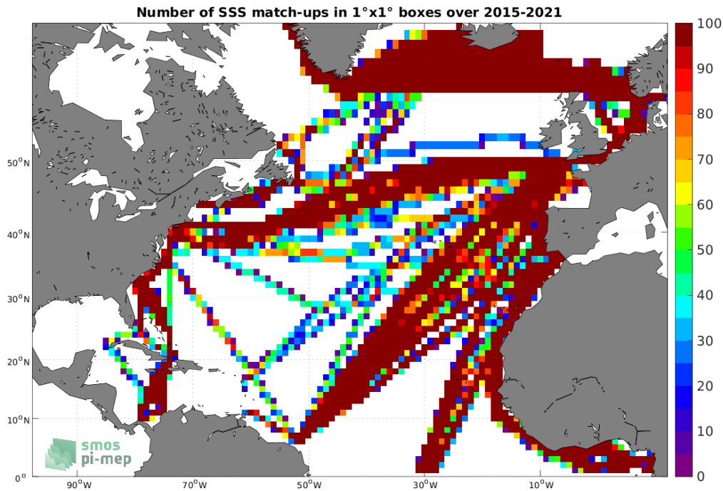
Figure 4: Number of SSS match-ups between TSG (LEGOS-DM) SSS and the SMAP SSS L3 v5.0 - Monthly (JPL) SSS product for the North Atlantic Ocean Pi-MEP region over 1^\circ \times 1^\circ boxes and for the full satellite product period.
