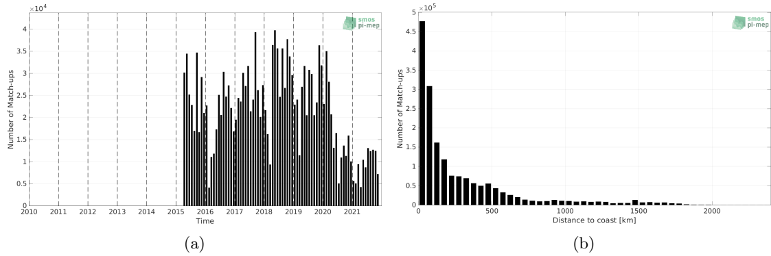
Figure 1: Number of match-ups between TSG (LEGOS-DM) and SMAP SSS L3 v5.0 - Monthly (JPL) SSS as a function of time (a) and as function of the distance to coast (b) over the North Atlantic Ocean Pi-MEP region and for the full satellite product period.
