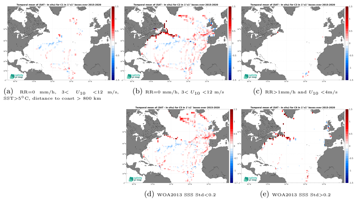
Figure 12: Temporal mean gridded over spatial boxes of size 1^\circ \times 1^\circ of \Delta\text{SSS} (SMAP SSS L3 v5.0 - Monthly (JPL) - TSG (GOSUD-Sailing-ship)) for 5 different subdatasets corresponding to:RR=0 mm/h, 3 < U_{10} < 12 m/s, SST >5^\circ\text{C} , distance to coast > 800 km (a), RR=0 mm/h, 3 < U_{10} < 12 m/s (b), RR >1 mm/h and U_{10} < 4 m/s (c), WOA2013 SSS Std <0.2 (d), WOA2013 SSS Std >0.2 (e).
