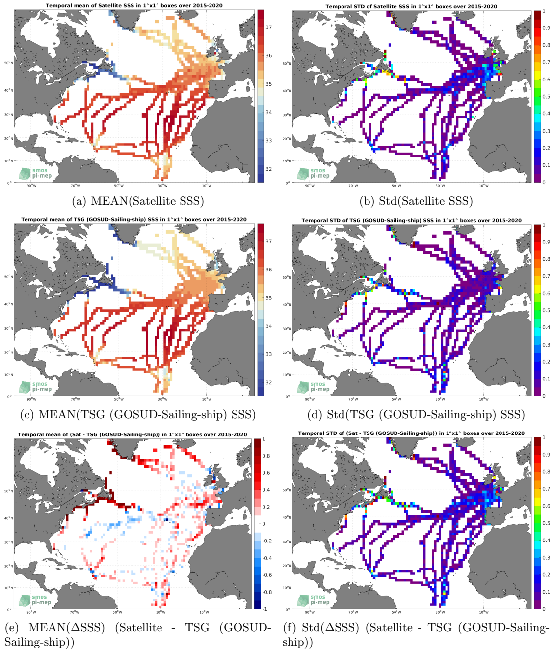
Figure 6: Temporal mean (left) and Std (right) of SSS from SMAP SSS L3 v5.0 - Monthly (JPL) (top), TSG (GOSUD-Sailing-ship) (middle), and of \Delta SSS (Satellite - TSG (GOSUD-Sailing-ship)). Only match-up pairs are used to generate these maps.
