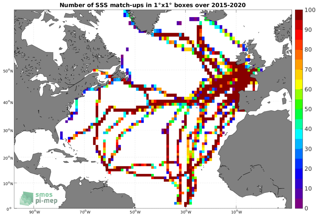
Figure 4: Number of SSS match-ups between TSG (GOSUD-Sailing-ship) SSS and the SMAP SSS L3 v5.0 - Monthly (JPL) SSS product for the North Atlantic Ocean Pi-MEP region over 1^\circ \times 1^\circ boxes and for the full satellite product period.
