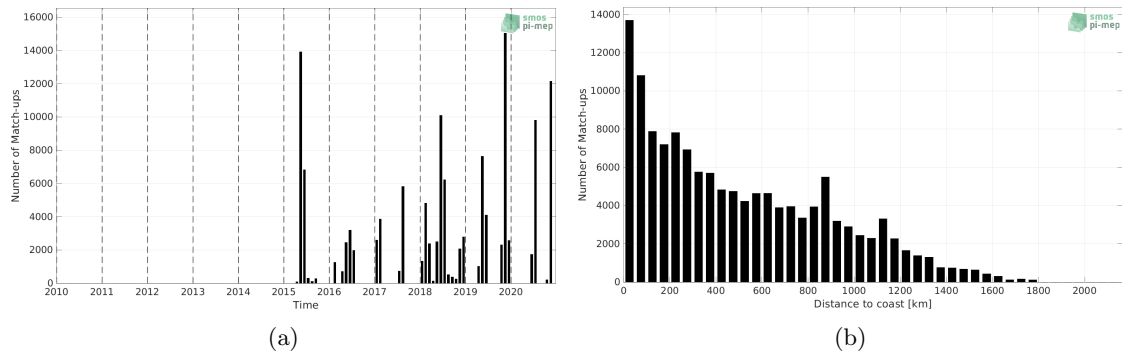
Figure 1: Number of match-ups between TSG (GOSUD-Sailing-ship) and SMAP SSS L3 v5.0 - Monthly (JPL) SSS as a function of time (a) and as function of the distance to coast (b) over the North Atlantic Ocean Pi-MEP region and for the full satellite product period.
