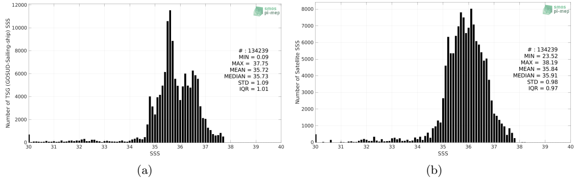
Figure 2: Histograms of SSS from TSG (GOSUD-Sailing-ship) (a) and SMAP SSS L3 v5.0 - Monthly (JPL) (b) considering all match-up pairs per bins of 0.1 over the North Atlantic Ocean Pi-MEP region and for the full satellite product period.
