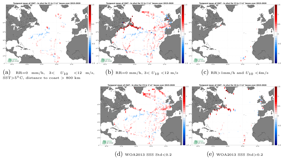
Figure 12: Temporal mean gridded over spatial boxes of size 1^\circ \times 1^\circ of \Delta SSS (SMAP SSS L3 v5.0 - Monthly (JPL) - TSG (GOSUD-Sailing-ship)) for 5 different subdatasets corresponding to:RR=0 mm/h, 3 < U_{10} < 12 m/s, SST>5°C, distance to coast > 800 km (a), RR=0 mm/h, 3 < U_{10} < 12 m/s (b), RR>1mm/h and U_{10} < 4 m/s (c), WOA2013 SSS Std<0.2 (d), WOA2013 SSS Std>0.2 (e).
