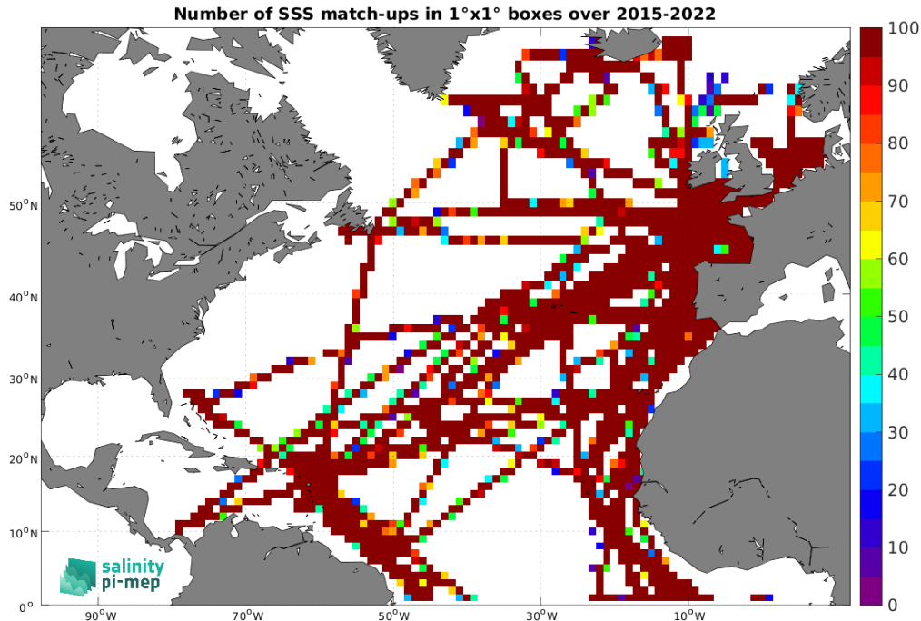
Figure 5: Number of SSS match-ups between TSG (GOSUD-Research-vessel) SSS and the SMAP SSS L3 v5.0 - Monthly (JPL) SSS product for the North Atlantic Ocean Pi-MEP region over 1^\circ \times 1^\circ boxes and for the full satellite product period.
