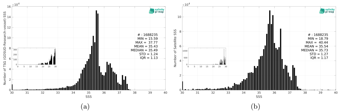
Figure 3: Histograms of SSS from TSG (GOSUD-Research-vessel) (a) and SMAP SSS L3 v5.0 - Monthly (JPL) (b) considering all match-up pairs per bins of 0.1 over the North Atlantic Ocean Pi-MEP region and for the full satellite product period.
