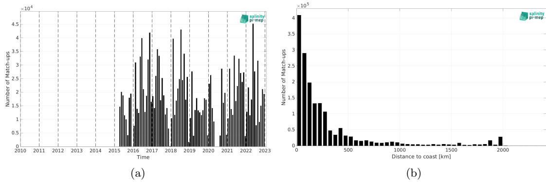
Figure 2: Number of match-ups between TSG (GOSUD-Research-vessel) and SMAP SSS L3 v5.0 - Monthly (JPL) SSS as a function of time (a) and as function of the distance to coast (b) over the North Atlantic Ocean Pi-MEP region and for the full satellite product period.
