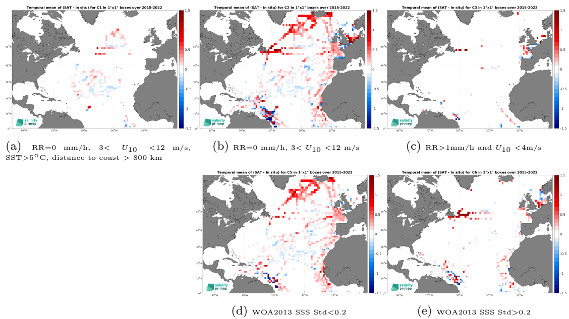
Figure 14: Temporal mean gridded over spatial boxes of size 1^\circ \times 1^\circ of \Delta\text{SSS} (SMAP SSS L3 v5.0 - Monthly (JPL) - TSG (GOSUD-Research-vessel)) for 5 different subdatasets corresponding to:RR=0 mm/h, 3 < U_{10} < 12 m/s, SST >5^\circ\text{C} , distance to coast > 800 km (a), RR=0 mm/h, 3 < U_{10} < 12 m/s (b), RR >1 mm/h and U_{10} < 4 m/s (c), WOA2013 SSS Std <0.2 (d), WOA2013 SSS Std >0.2 (e).
