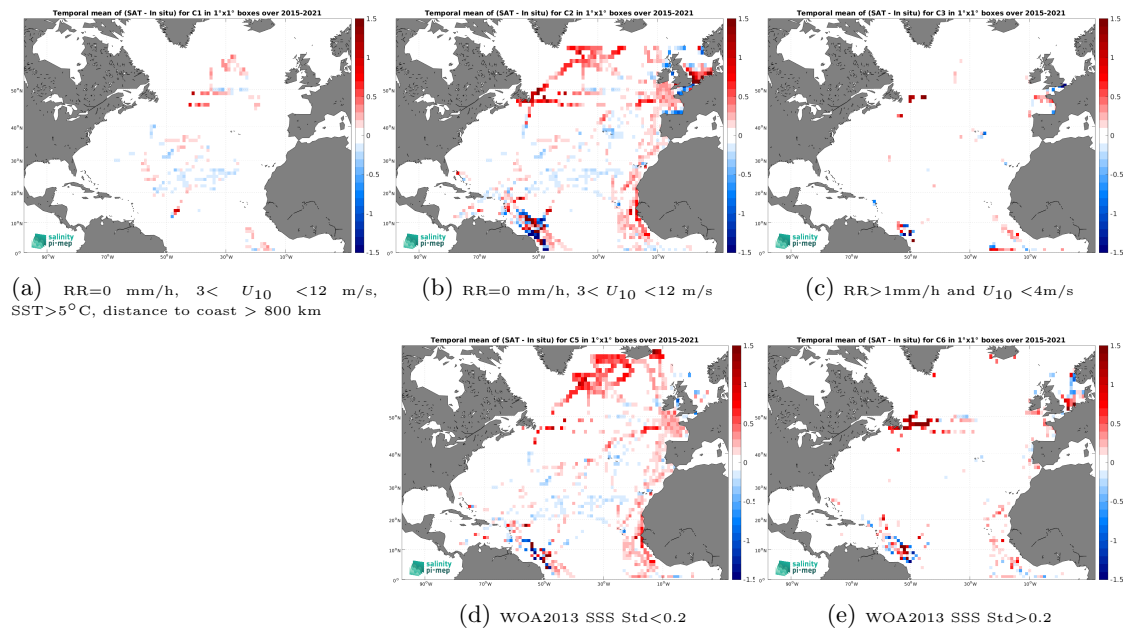
Figure 12: Temporal mean gridded over spatial boxes of size 1^\circ \times 1^\circ of \Delta\text{SSS} (SMAP SSS L3 v5.0 - Monthly (JPL) - TSG (GOSUD-Research-vessel)) for 5 different subdatasets corresponding to:RR=0 mm/h, 3 < U_{10} < 12 m/s, SST >5^\circ\text{C} , distance to coast > 800 km (a), RR=0 mm/h, 3 < U_{10} < 12 m/s (b), RR >1 mm/h and U_{10} < 4 m/s (c), WOA2013 SSS Std <0.2 (d), WOA2013 SSS Std >0.2 (e).
