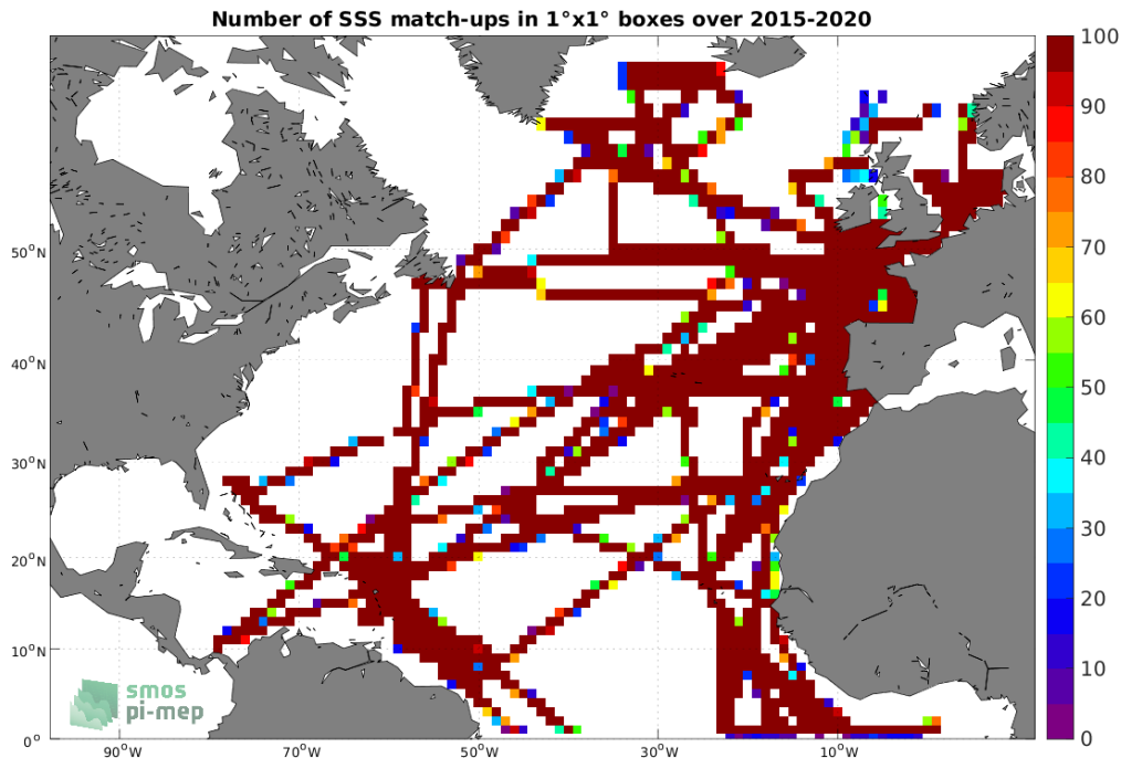
Figure 4: Number of SSS match-ups between TSG (GOSUD-Research-vessel) SSS and the SMAP SSS L3 v5.0 - Monthly (JPL) SSS product for the North Atlantic Ocean Pi-MEP region over 1°x1° boxes and for the full satellite product period.
