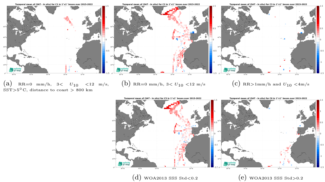
Figure 14: Temporal mean gridded over spatial boxes of size 1^\circ \times 1^\circ of \Delta\text{SSS} (SMAP SSS L3 v5.0 - Monthly (JPL) - TSG (CSIC-UTM)) for 5 different subdatasets corresponding to:RR=0 mm/h, 3 < U_{10} < 12 m/s, SST >5^\circ\text{C} , distance to coast > 800 km (a), RR=0 mm/h, 3 < U_{10} < 12 m/s (b), RR >1 mm/h and U_{10} < 4 m/s (c), WOA2013 SSS Std <0.2 (d), WOA2013 SSS Std >0.2 (e).
