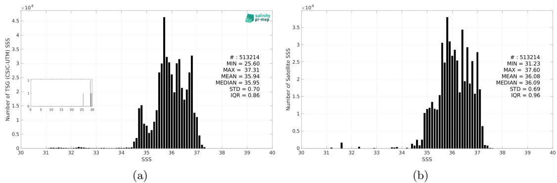
Figure 3: Histograms of SSS from TSG (CSIC-UTM) (a) and SMAP SSS L3 v5.0 - Monthly (JPL) (b) considering all match-up pairs per bins of 0.1 over the North Atlantic Ocean Pi-MEP region and for the full satellite product period.
