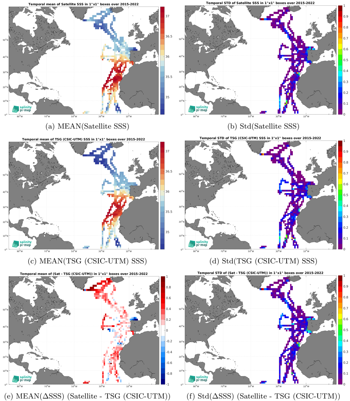
Figure 7: Temporal mean (left) and Std (right) of SSS from SMAP SSS L3 v5.0 - Monthly (JPL) (top), TSG (CSIC-UTM) (middle), and of \Delta SSS (Satellite - TSG (CSIC-UTM)). Only match-up pairs are used to generate these maps.
