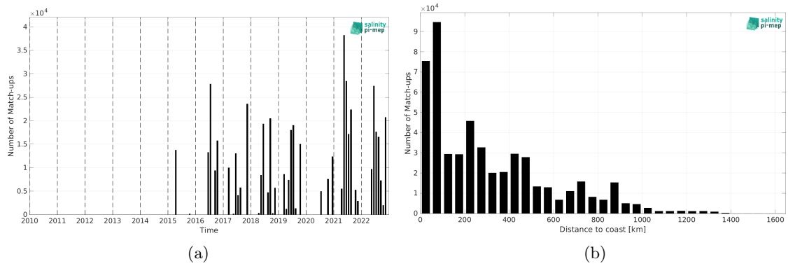
Figure 2: Number of match-ups between TSG (CSIC-UTM) and SMAP SSS L3 v5.0 - Monthly (JPL) SSS as a function of time (a) and as function of the distance to coast (b) over the North Atlantic Ocean Pi-MEP region and for the full satellite product period.
