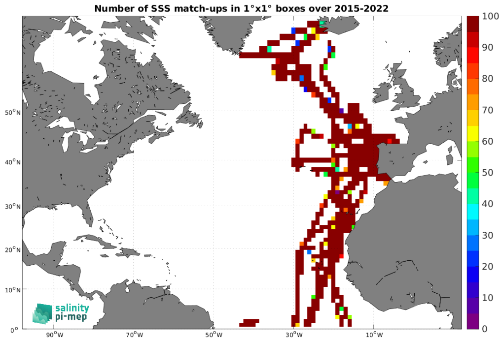
Figure 5: Number of SSS match-ups between TSG (CSIC-UTM) SSS and the SMAP SSS L3 v5.0 - Monthly (JPL) SSS product for the North Atlantic Ocean Pi-MEP region over 1^\circ \times 1^\circ boxes and for the full satellite product period.
