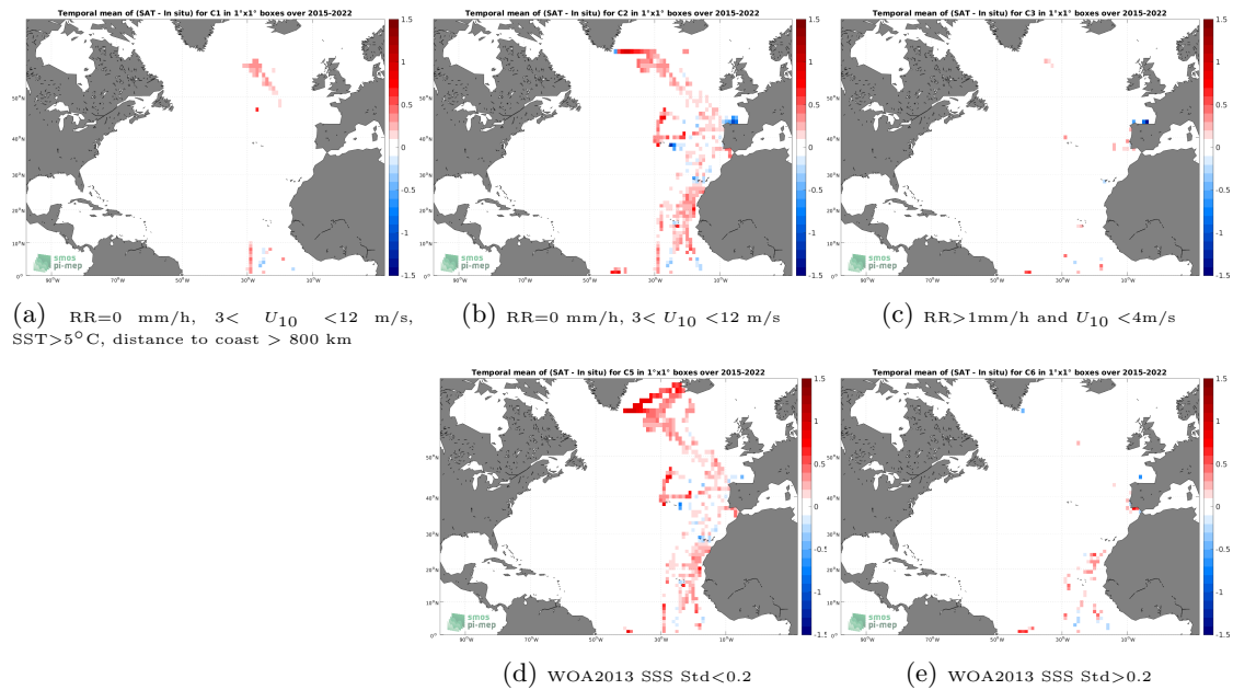
Figure 12: Temporal mean gridded over spatial boxes of size 1^\circ \times 1^\circ of \Delta\text{SSS} (SMAP SSS L3 v5.0 - Monthly (JPL) - TSG (CSIC-UTM)) for 5 different subdatasets corresponding to:RR=0 mm/h, 3 < U_{10} < 12 m/s, SST >5^\circ\text{C} , distance to coast > 800 km (a), RR=0 mm/h, 3 < U_{10} < 12 m/s (b), RR >1 mm/h and U_{10} < 4 m/s (c), WOA2013 SSS Std <0.2 (d), WOA2013 SSS Std >0.2 (e).
