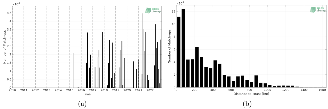
Figure 1: Number of match-ups between TSG (CSIC-UTM) and SMAP SSS L3 v5.0 - Monthly (JPL) SSS as a function of time (a) and as function of the distance to coast (b) over the North Atlantic Ocean Pi-MEP region and for the full satellite product period.
