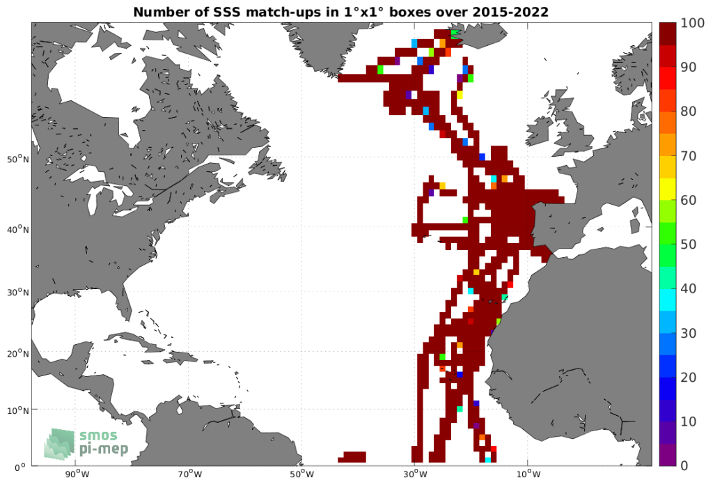
Figure 4: Number of SSS match-ups between TSG (CSIC-UTM) SSS and the SMAP SSS L3 v5.0 - Monthly (JPL) SSS product for the North Atlantic Ocean Pi-MEP region over 1^\circ \times 1^\circ boxes and for the full satellite product period.
