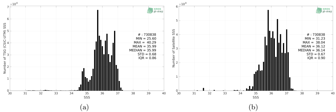
Figure 2: Histograms of SSS from TSG (CSIC-UTM) (a) and SMAP SSS L3 v5.0 - Monthly (JPL) (b) considering all match-up pairs per bins of 0.1 over the North Atlantic Ocean Pi-MEP region and for the full satellite product period.
