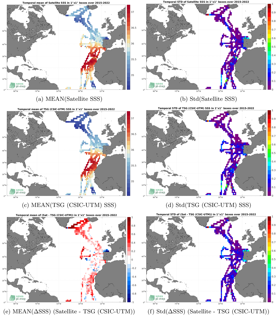
Figure 6: Temporal mean (left) and Std (right) of SSS from SMAP SSS L3 v5.0 - Monthly (JPL) (top), TSG (CSIC-UTM) (middle), and of \Delta SSS (Satellite - TSG (CSIC-UTM)). Only match-up pairs are used to generate these maps.
