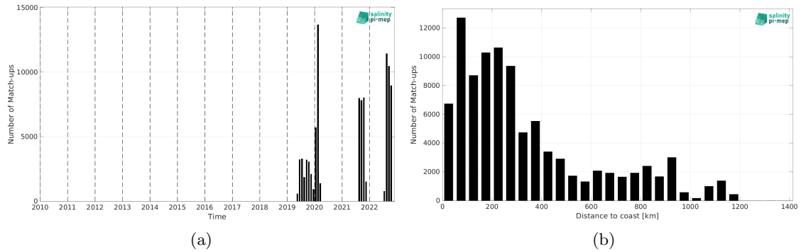
Figure 2: Number of match-ups between Saildrone and SMAP SSS L3 v5.0 - Monthly (JPL) SSS as a function of time (a) and as function of the distance to coast (b) over the North Atlantic Ocean Pi-MEP region and for the full satellite product period.
