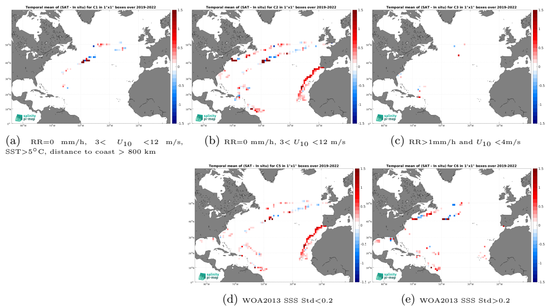
Figure 14: Temporal mean gridded over spatial boxes of size 1^\circ \times 1^\circ of \Delta\text{SSS} (SMAP SSS L3 v5.0 - Monthly (JPL) - Sairdrone) for 5 different subdatasets corresponding to:RR=0 mm/h, 3 < U_{10} < 12 m/s, SST > 5°C, distance to coast > 800 km (a), RR=0 mm/h, 3 < U_{10} < 12 m/s (b), RR > 1mm/h and U_{10} < 4 m/s (c), WOA2013 SSS Std < 0.2 (d), WOA2013 SSS Std > 0.2 (e).
