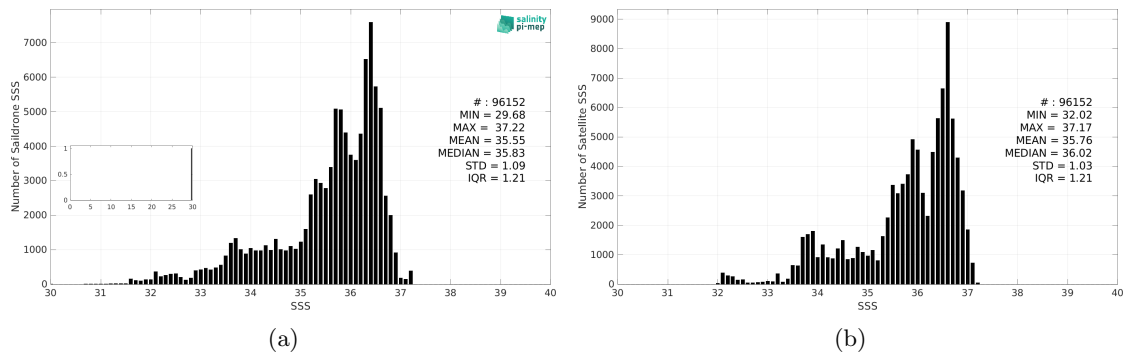
Figure 3: Histograms of SSS from Saildrone (a) and SMAP SSS L3 v5.0 - Monthly (JPL) (b) considering all match-up pairs per bins of 0.1 over the North Atlantic Ocean Pi-MEP region and for the full satellite product period.
