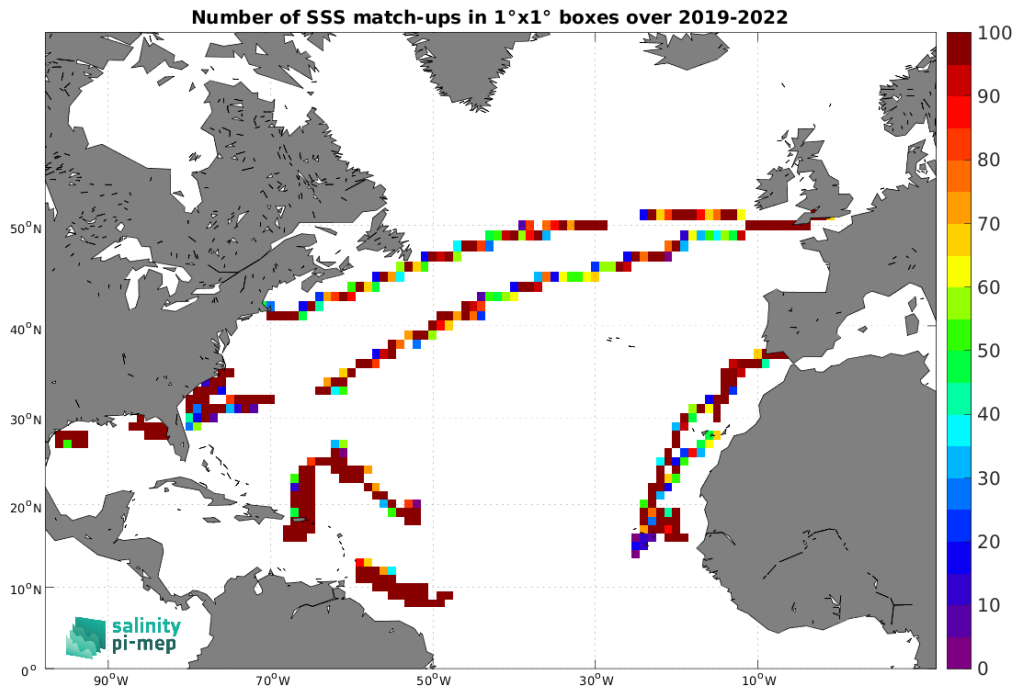
Figure 5: Number of SSS match-ups between Saildrone SSS and the SMAP SSS L3 v5.0 - Monthly (JPL) SSS product for the North Atlantic Ocean Pi-MEP region over 1^\circ \times 1^\circ boxes and for the full satellite product period.
