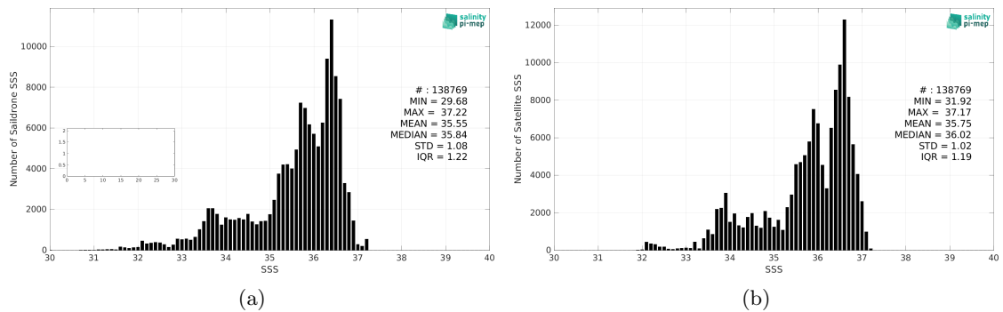
Figure 2: Histograms of SSS from Saildrone (a) and SMAP SSS L3 v5.0 - Monthly (JPL) (b) considering all match-up pairs per bins of 0.1 over the North Atlantic Ocean Pi-MEP region and for the full satellite product period.
