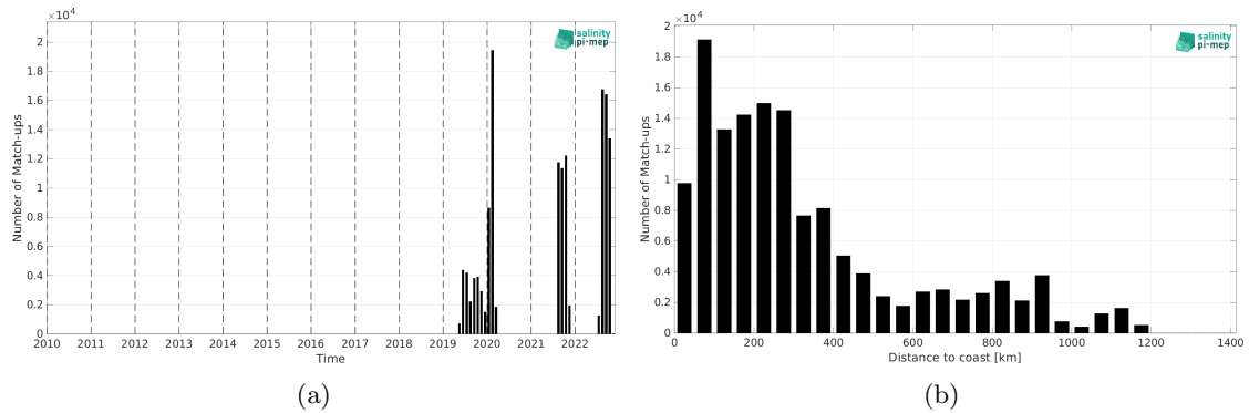
Figure 1: Number of match-ups between Saildrone and SMAP SSS L3 v5.0 - Monthly (JPL) SSS as a function of time (a) and as function of the distance to coast (b) over the North Atlantic Ocean Pi-MEP region and for the full satellite product period.
