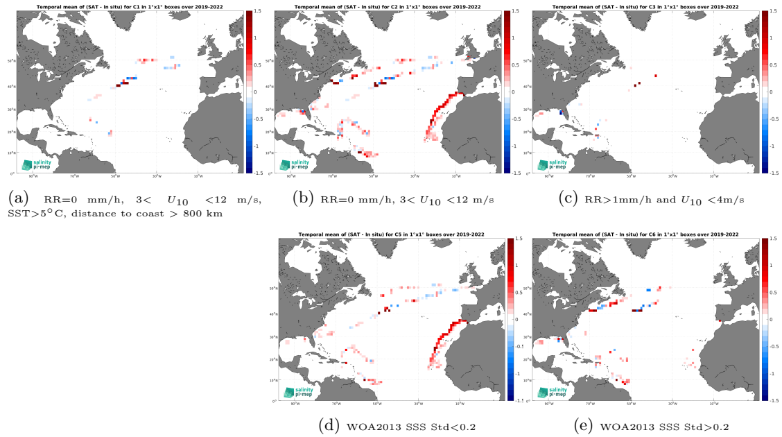
Figure 12: Temporal mean gridded over spatial boxes of size 1^\circ \times 1^\circ of \Delta SSS (SMAP SSS L3 v5.0 - Monthly (JPL) - Sairdrone) for 5 different subdatasets corresponding to:RR=0 mm/h, 3 < U_{10} < 12 m/s, SST >5^\circ\text{C} , distance to coast > 800 km (a), RR=0 mm/h, 3 < U_{10} < 12 m/s (b), RR >1 mm/h and U_{10} < 4 m/s (c), WOA2013 SSS Std <0.2 (d), WOA2013 SSS Std >0.2 (e).
