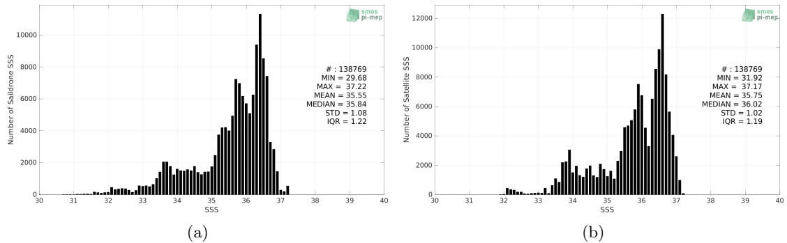
Figure 2: Histograms of SSS from Sairdrone (a) and SMAP SSS L3 v5.0 - Monthly (JPL) (b) considering all match-up pairs per bins of 0.1 over the North Atlantic Ocean Pi-MEP region and for the full satellite product period.
