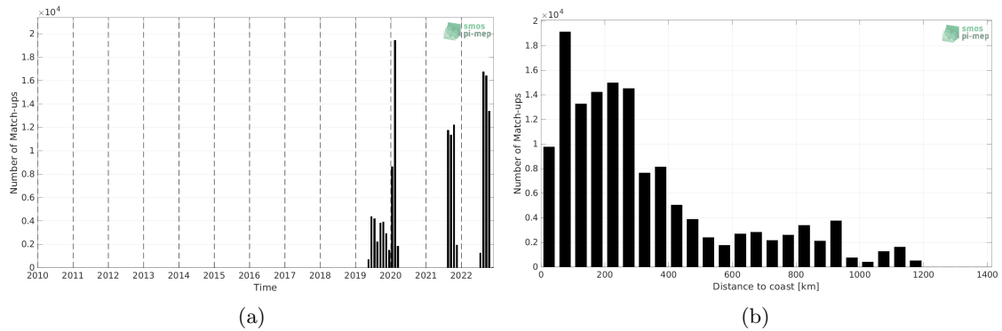
Figure 1: Number of match-ups between Sairdrone and SMAP SSS L3 v5.0 - Monthly (JPL) SSS as a function of time (a) and as function of the distance to coast (b) over the North Atlantic Ocean Pi-MEP region and for the full satellite product period.
