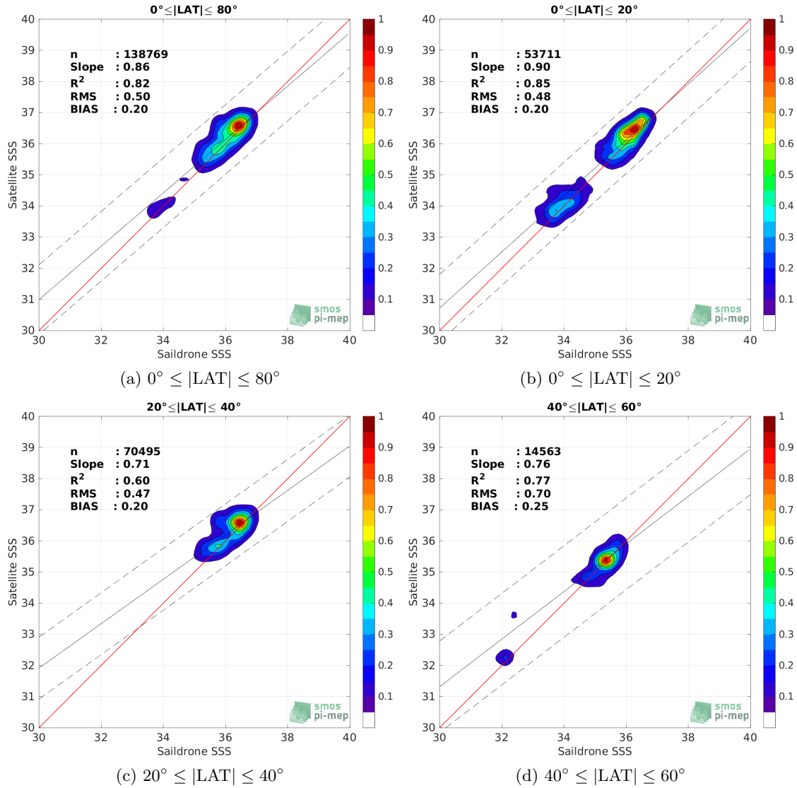
Figure 9: Contour maps of the concentration of SMAP SSS L3 v5.0 - Monthly (JPL) SSS (y-axis) versus Saildrone SSS (x-axis) at match-up pairs for different latitude bands. For each plot, the red line shows x=y . The black thin and dashed lines indicate a linear fit through the data cloud and the \pm 95\% confidence levels, respectively. The number match-up pairs n , the slope and R^2 coefficient of the linear fit, the root mean square (RMS) and the mean bias between satellite and in situ data are indicated for each latitude band in each plots.
