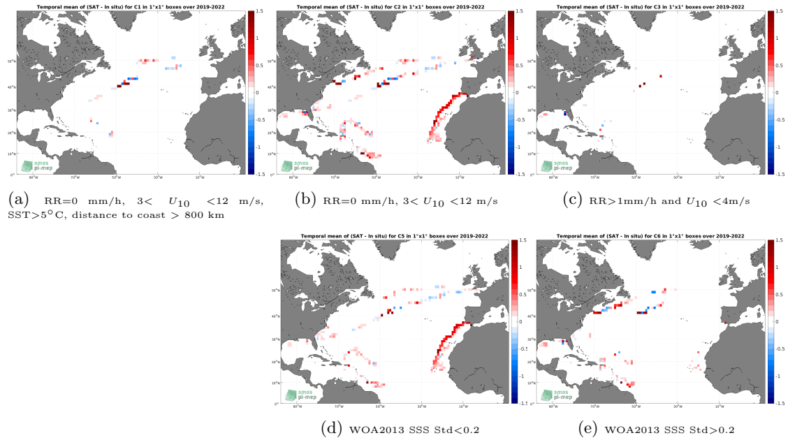
Figure 12: Temporal mean gridded over spatial boxes of size 1^\circ \times 1^\circ of \Delta\text{SSS} (SMAP SSS L3 v5.0 - Monthly (JPL) - Sairdrone) for 5 different subdatasets corresponding to:RR=0 mm/h, 3 < U_{10} < 12 m/s, SST >5^\circ\text{C} , distance to coast > 800 km (a), RR=0 mm/h, 3 < U_{10} < 12 m/s (b), RR >1 mm/h and U_{10} < 4 m/s (c), WOA2013 SSS Std <0.2 (d), WOA2013 SSS Std >0.2 (e).
