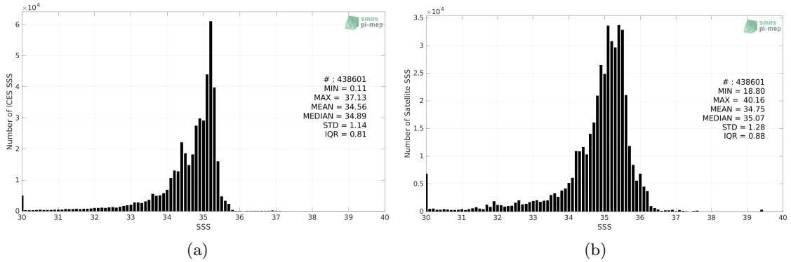
Figure 2: Histograms of SSS from ICES (a) and SMAP SSS L3 v5.0 - Monthly (JPL) (b) considering all match-up pairs per bins of 0.1 over the North Atlantic Ocean Pi-MEP region and for the full satellite product period.
