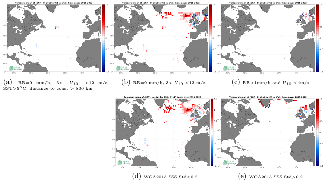
Figure 12: Temporal mean gridded over spatial boxes of size 1^\circ \times 1^\circ of \Delta\text{SSS} (SMAP SSS L3 v5.0 - Monthly (JPL) - ICES) for 5 different subdatasets corresponding to:RR=0 mm/h, 3 < U_{10} < 12 m/s, SST >5^\circ\text{C} , distance to coast > 800 km (a), RR=0 mm/h, 3 < U_{10} < 12 m/s (b), RR >1 mm/h and U_{10} < 4 m/s (c), WOA2013 SSS Std <0.2 (d), WOA2013 SSS Std >0.2 (e).
