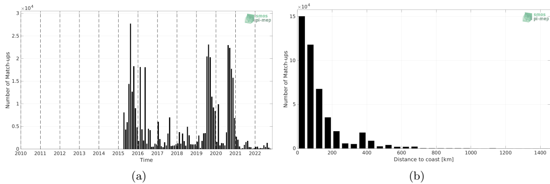
Figure 1: Number of match-ups between ICES and SMAP SSS L3 v5.0 - Monthly (JPL) SSS as a function of time (a) and as function of the distance to coast (b) over the North Atlantic Ocean Pi-MEP region and for the full satellite product period.
