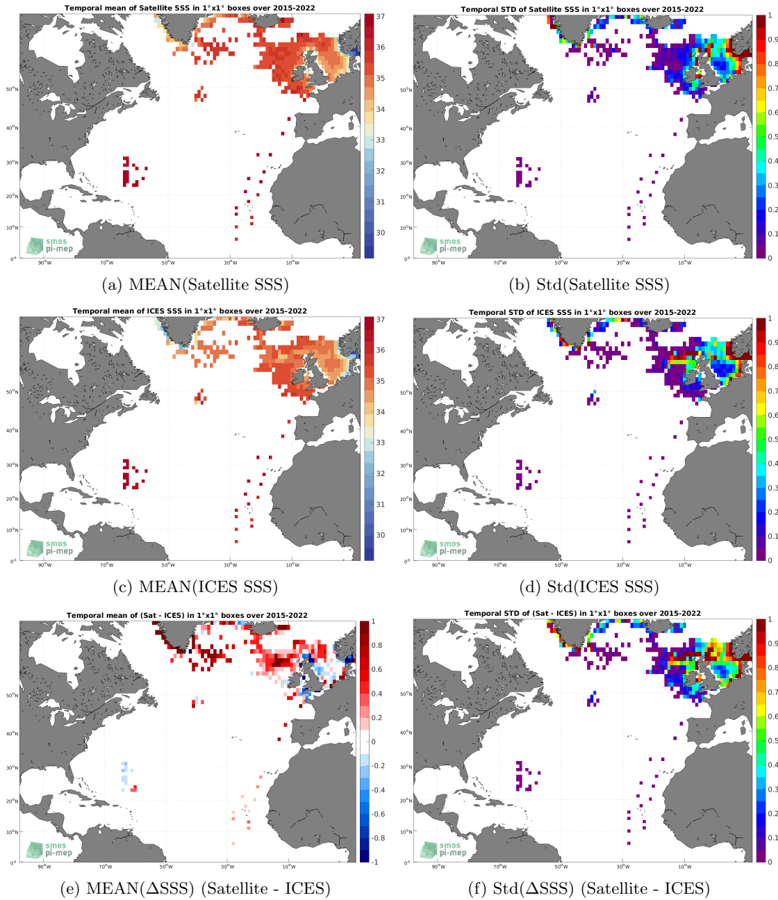
Figure 6: Temporal mean (left) and Std (right) of SSS from SMAP SSS L3 v5.0 - Monthly (JPL) (top), ICES (middle), and of \Delta SSS (Satellite - ICES). Only match-up pairs are used to generate these maps.
