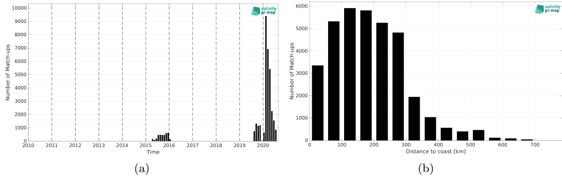
Figure 2: Number of match-ups between Surface drifters and SMAP SSS L3 v5.0 - Monthly (JPL) SSS as a function of time (a) and as function of the distance to coast (b) over the North Atlantic Ocean Pi-MEP region and for the full satellite product period.
