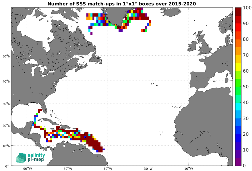
Figure 4: Number of SSS match-ups between Surface drifters SSS and the SMAP SSS L3 v5.0 - Monthly (JPL) SSS product for the North Atlantic Ocean Pi-MEP region over 1^\circ \times 1^\circ boxes and for the full satellite product period.
