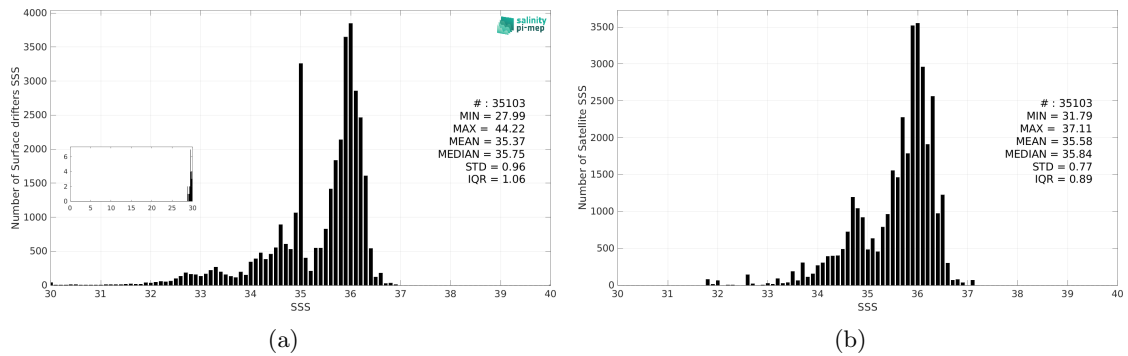
Figure 3: Histograms of SSS from Surface drifters (a) and SMAP SSS L3 v5.0 - Monthly (JPL) (b) considering all match-up pairs per bins of 0.1 over the North Atlantic Ocean Pi-MEP region and for the full satellite product period.
