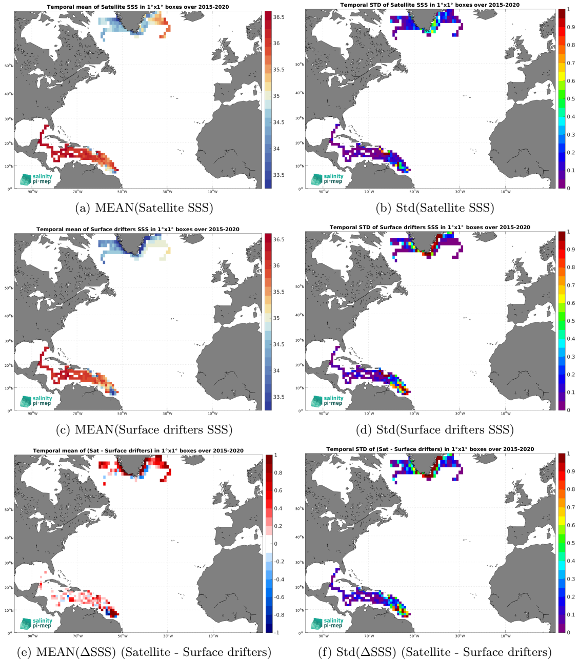
Figure 6: Temporal mean (left) and Std (right) of SSS from SMAP SSS L3 v5.0 - Monthly (JPL) (top), Surface drifters (middle), and of \Delta SSS (Satellite - Surface drifters). Only match-up pairs are used to generate these maps.
