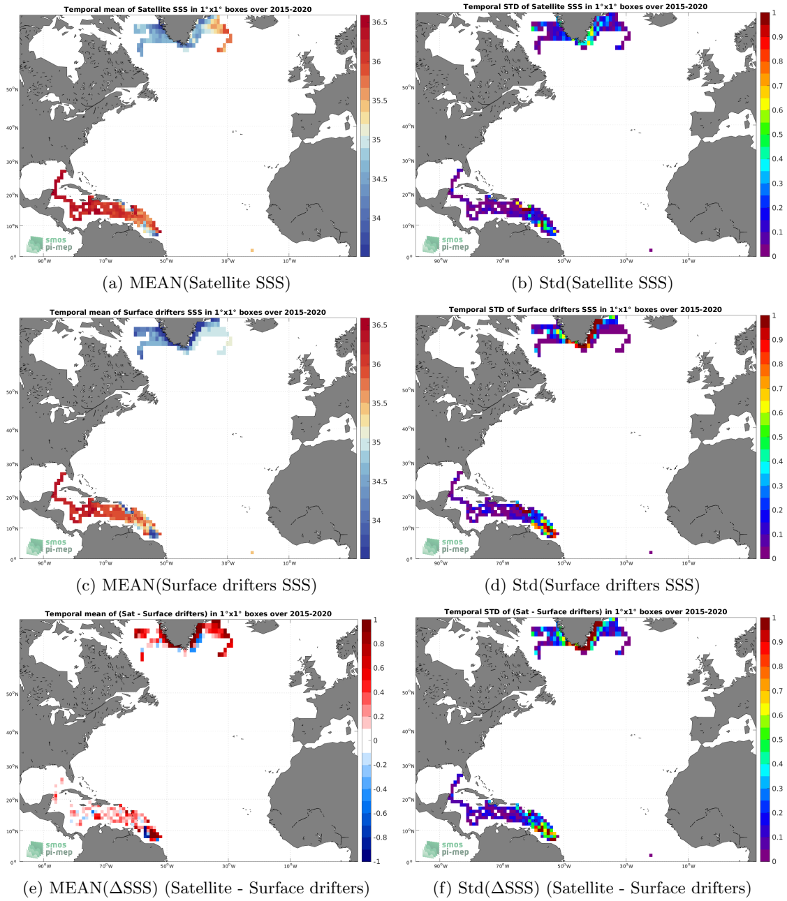
Figure 5: Temporal mean (left) and Std (right) of SSS from SMAP SSS L3 v5.0 - Monthly (JPL) (top), Surface drifters (middle), and of \Delta SSS (Satellite - Surface drifters). Only match-up pairs are used to generate these maps.
