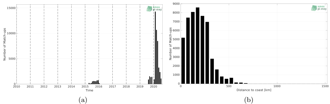
Figure 1: Number of match-ups between Surface drifters and SMAP SSS L3 v5.0 - Monthly (JPL) SSS as a function of time (a) and as function of the distance to coast (b) over the North Atlantic Ocean Pi-MEP region and for the full satellite product period.
