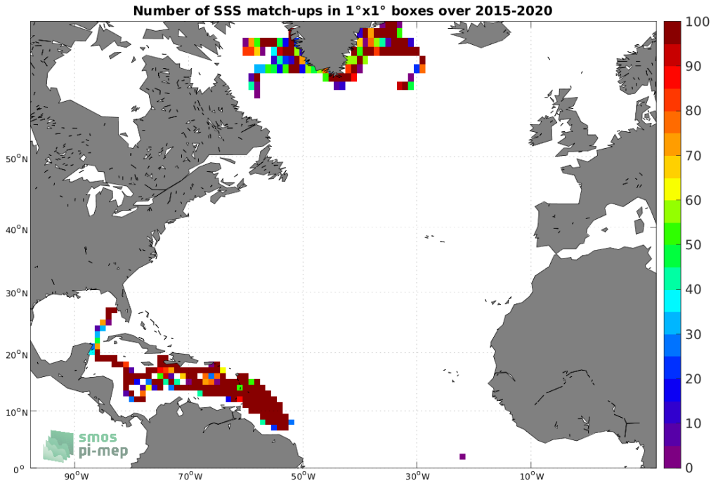
Figure 3: Number of SSS match-ups between Surface drifters SSS and the SMAP SSS L3 v5.0 - Monthly (JPL) SSS product for the North Atlantic Ocean Pi-MEP region over 1^\circ \times 1^\circ boxes and for the full satellite product period.
