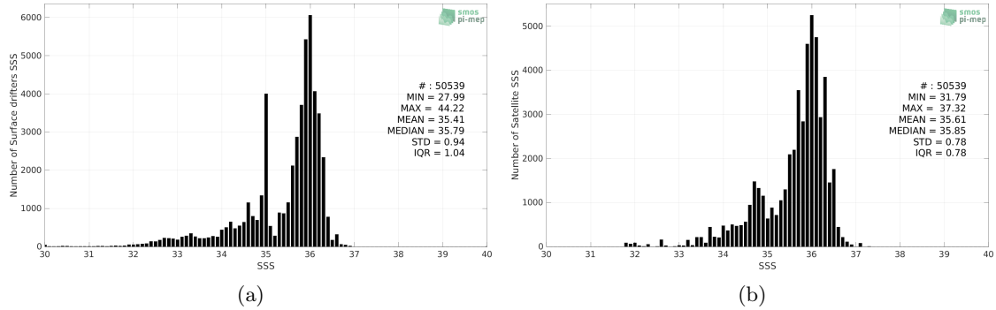
Figure 2: Histograms of SSS from Surface drifters (a) and SMAP SSS L3 v5.0 - Monthly (JPL) (b) considering all match-up pairs per bins of 0.1 over the North Atlantic Ocean Pi-MEP region and for the full satellite product period.
