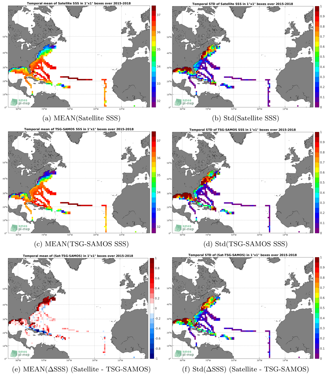
Figure 6: Temporal mean (left) and Std (right) of SSS from SMAP-L3-JPL-V4.2-8DAY-RUNNING-60KM (top), TSG-SAMOS (middle), and of \Delta SSS (Satellite - TSG-SAMOS). Only match-up pairs are used to generate these maps.
