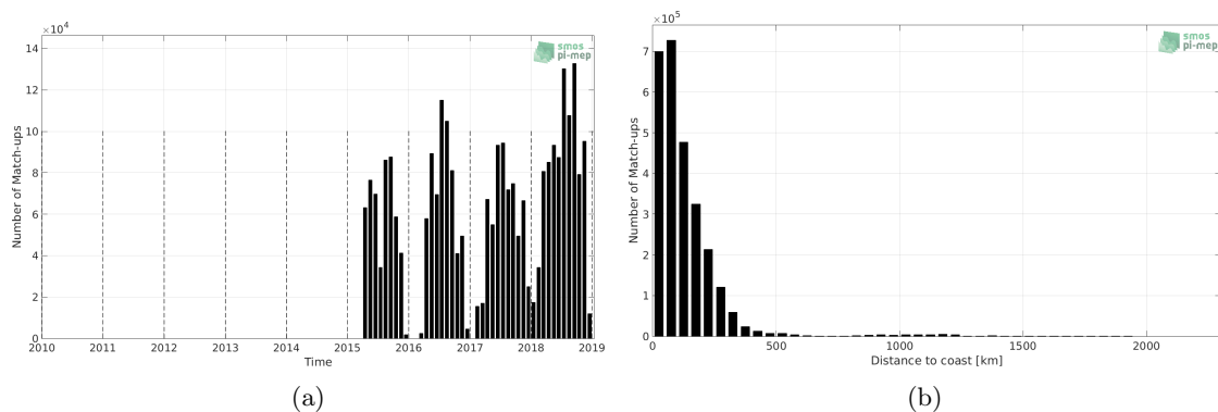
Figure 1: Number of match-ups between TSG-SAMOS and SMAP-L3-JPL-V4.2-8DAY-RUNNING-60KM SSS as a function of time (a) and as function of the distance to coast (b) over the North Atlantic Ocean Pi-MEP region and for the full satellite product period.
