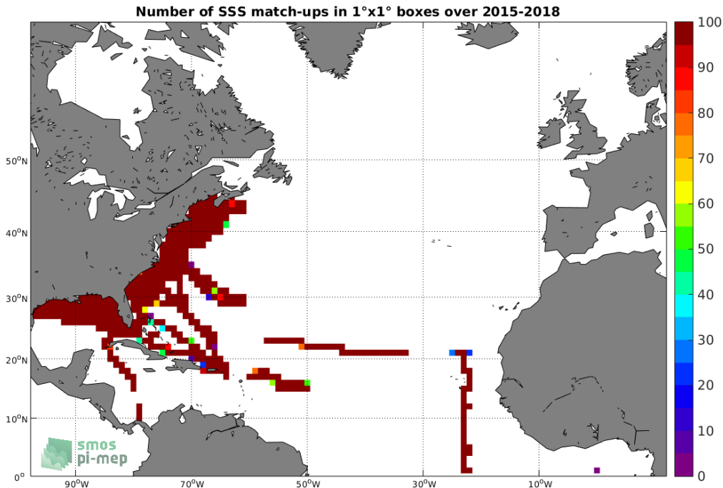
Figure 4: Number of SSS match-ups between TSG-SAMOS SSS and the SMAP-L3-JPL-V4.2-8DAY-RUNNING-60KM SSS product for the North Atlantic Ocean Pi-MEP region over 1^\circ \times 1^\circ boxes and for the full satellite product period.
