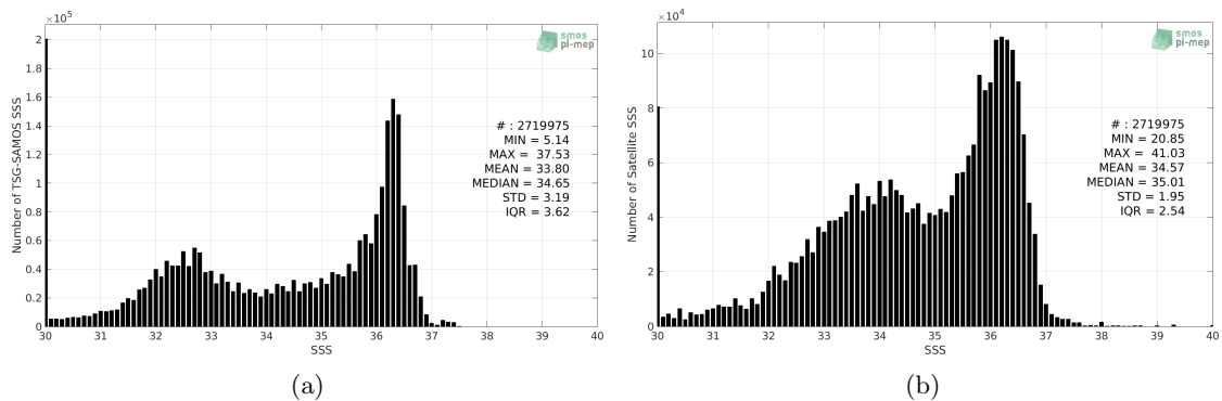
Figure 2: Histograms of SSS from TSG-SAMOS (a) and SMAP-L3-JPL-V4.2-8DAY-RUNNING-60KM (b) considering all match-up pairs per bins of 0.1 over the North Atlantic Ocean Pi-MEP region and for the full satellite product period.
