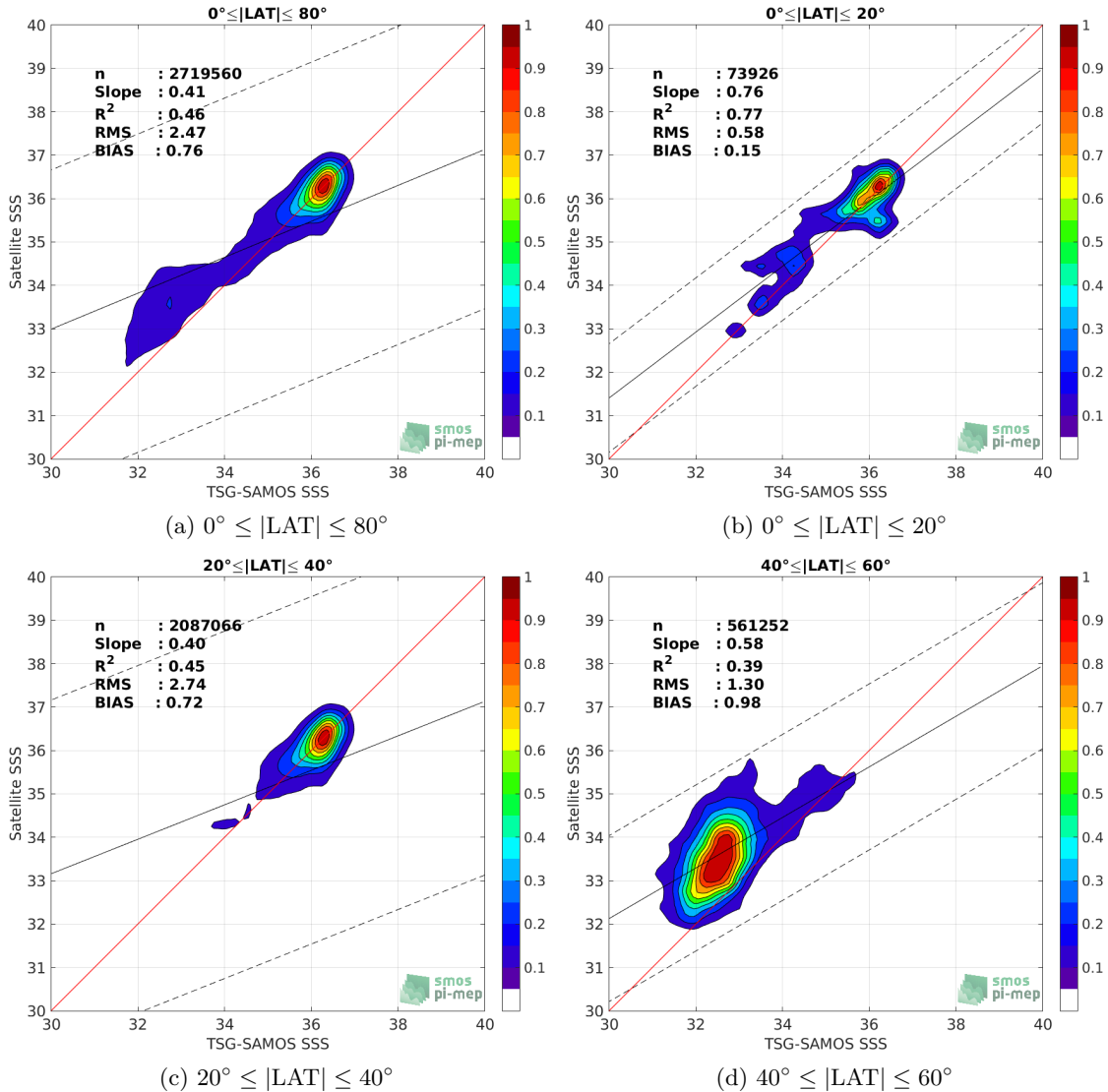
Figure 9: Contour maps of the concentration of SMAP-L3-JPL-V4.2-8DAY-RUNNING-60KM SSS (y-axis) versus TSG-SAMOS SSS (x-axis) at match-up pairs for different latitude bands. For each plot, the red line shows x=y . The black thin and dashed lines indicate a linear fit through the data cloud and the \pm 95\% confidence levels, respectively. The number match-up pairs n , the slope and R^2 coefficient of the linear fit, the root mean square (RMS) and the mean bias between satellite and in situ data are indicated for each latitude band in each plots.
