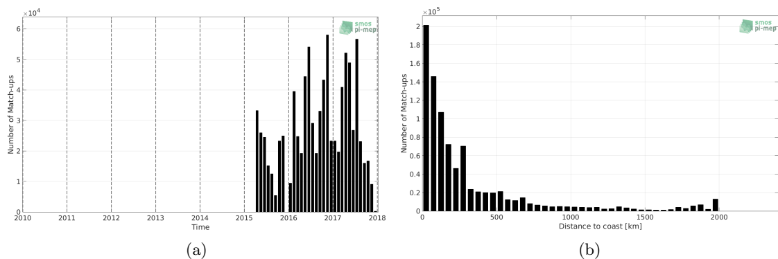
Figure 1: Number of match-ups between TSG-GOSUD-Research-vessel and SMAP-L3-JPL-V4.2-8DAY-RUNNING-60KM SSS as a function of time (a) and as function of the distance to coast (b) over the North Atlantic Ocean Pi-MEP region and for the full satellite product period.
