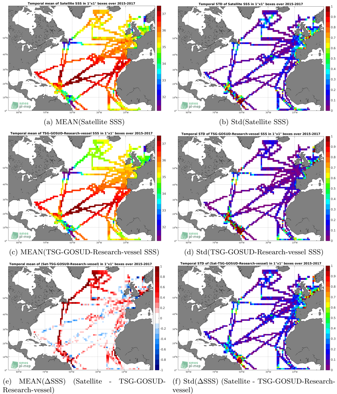
Figure 6: Temporal mean (left) and Std (right) of SSS from SMAP-L3-JPL-V4.2-8DAY-RUNNING-60KM (top), TSG-GOSUD-Research-vessel (middle), and of \Delta SSS (Satellite - TSG-GOSUD-Research-vessel). Only match-up pairs are used to generate these maps.
