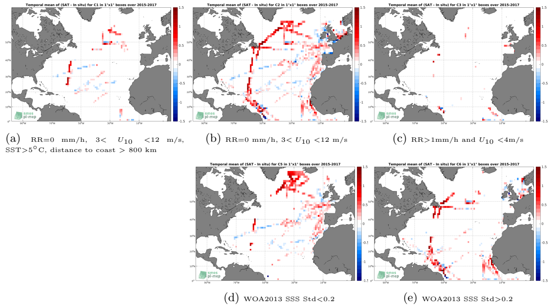
Figure 12: Temporal mean gridded over spatial boxes of size 1^\circ \times 1^\circ of \Delta SSS (SMAP-L3-JPL-V4.2-8DAY-RUNNING-60KM - TSG-GOSUD-Research-vessel) for 5 different subdatasets corresponding to:RR=0 mm/h, 3 < U_{10} < 12 m/s, SST >5^\circ C, distance to coast > 800 km (a), RR=0 mm/h, 3 < U_{10} < 12 m/s (b), RR >1 mm/h and U_{10} < 4 m/s (c), WOA2013 SSS Std <0.2 (d), WOA2013 SSS Std >0.2 (e).
