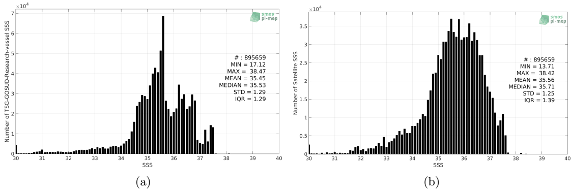
Figure 2: Histograms of SSS from TSG-GOSUD-Research-vessel (a) and SMAP-L3-JPL-V4.2-8DAY-RUNNING-60KM (b) considering all match-up pairs per bins of 0.1 over the North Atlantic Ocean Pi-MEP region and for the full satellite product period.
