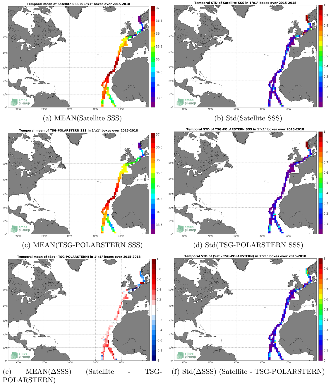
Figure 6: Temporal mean (left) and Std (right) of SSS from SMAP-L3-JPL-V4.2-MONTHLY-60KM (top), TSG-POLARSTERN (middle), and of \Delta SSS (Satellite - TSG-POLARSTERN). Only match-up pairs are used to generate these maps.
