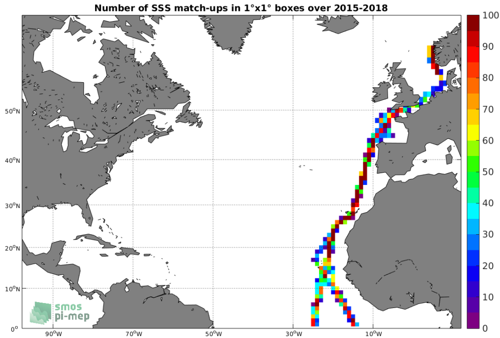
Figure 4: Number of SSS match-ups between TSG-POLARSTERN SSS and the SMAP-L3-JPL-V4.2-MONTHLY-60KM SSS product for the North Atlantic Ocean Pi-MEP region over 1^\circ \times 1^\circ boxes and for the full satellite product period.
