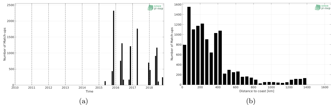
Figure 1: Number of match-ups between TSG-POLARSTERN and SMAP-L3-JPL-V4.2-MONTHLY-60KM SSS as a function of time (a) and as function of the distance to coast (b) over the North Atlantic Ocean Pi-MEP region and for the full satellite product period.
