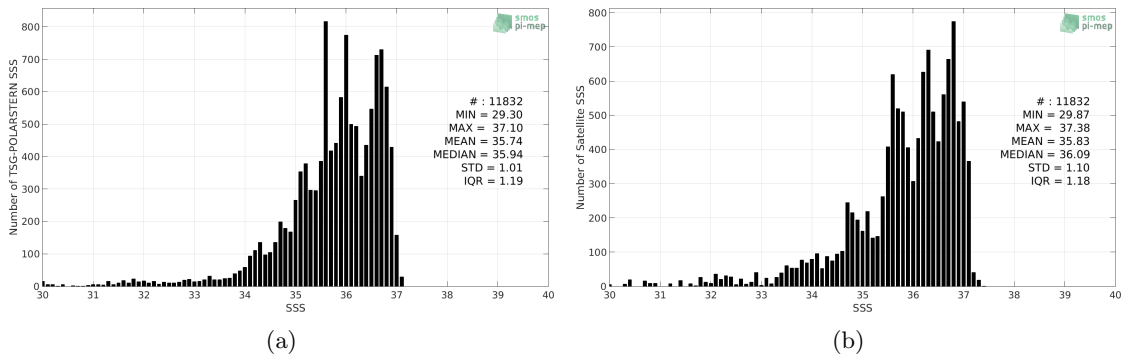
Figure 2: Histograms of SSS from TSG-POLARSTERN (a) and SMAP-L3-JPL-V4.2-MONTHLY-60KM (b) considering all match-up pairs per bins of 0.1 over the North Atlantic Ocean Pi-MEP region and for the full satellite product period.
