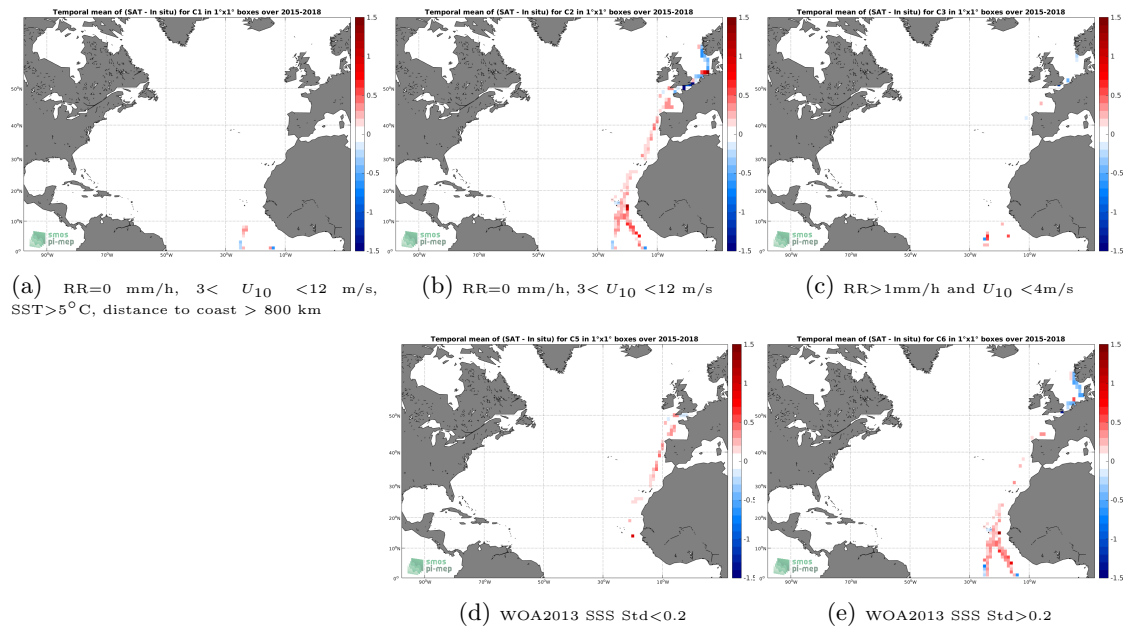
Figure 12: Temporal mean gridded over spatial boxes of size 1^\circ \times 1^\circ of \Delta SSS (SMAP-L3-JPL-V4.2-MONTHLY-60KM - TSG-POLARSTERN) for 5 different subdatasets corresponding to:RR=0 mm/h, 3 < U_{10} < 12 m/s, SST > 5^\circ\text{C} , distance to coast > 800 km (a), RR=0 mm/h, 3 < U_{10} < 12 m/s (b), RR > 1 mm/h and U_{10} < 4 m/s (c), WOA2013 SSS Std < 0.2 (d), WOA2013 SSS Std > 0.2 (e).
