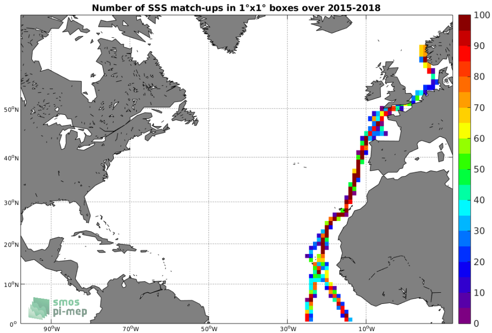
Figure 4: Number of SSS match-ups between TSG-POLARSTERN SSS and the SMAP-L3-JPL-V4.2-MONTHLY-60KM SSS product for the North Atlantic Ocean Pi-MEP region over 1°x1° boxes and for the full satellite product period.
