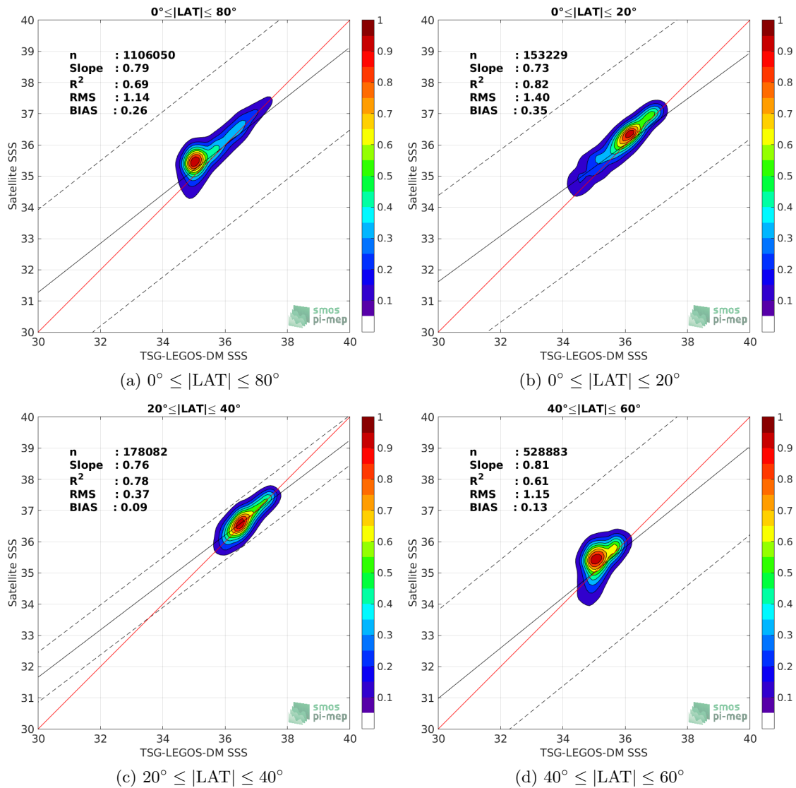
Figure 9: Contour maps of the concentration of SMAP-L3-JPL-V4.2-MONTHLY-60KM SSS (y-axis) versus TSG-LEGOS-DM SSS (x-axis) at match-up pairs for different latitude bands. For each plot, the red line shows x=y . The black thin and dashed lines indicate a linear fit through the data cloud and the \pm 95\% confidence levels, respectively. The number match-up pairs n , the slope and R^2 coefficient of the linear fit, the root mean square (RMS) and the mean bias between satellite and in situ data are indicated for each latitude band in each plots.
