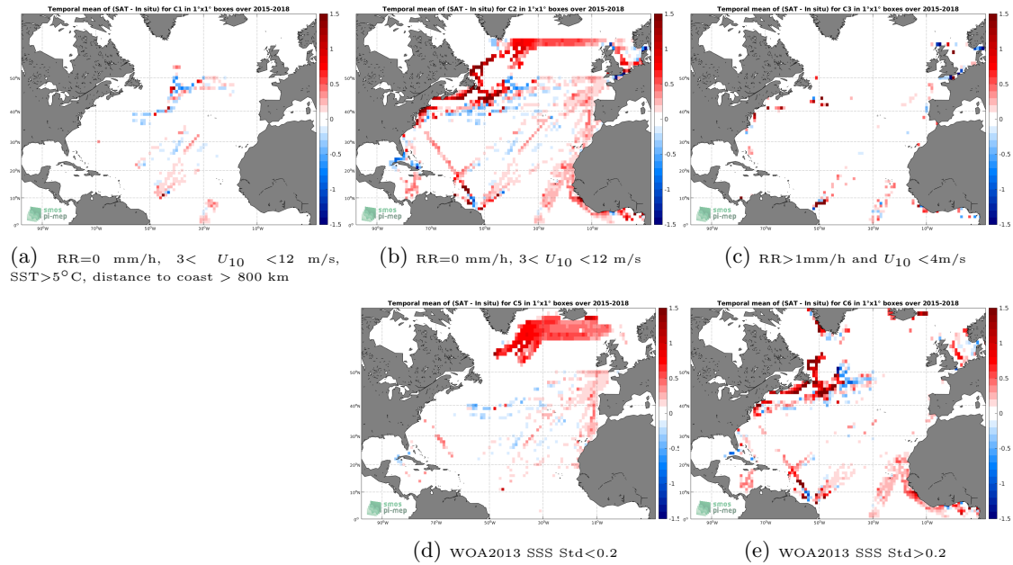
Figure 12: Temporal mean gridded over spatial boxes of size 1^\circ \times 1^\circ of \Delta SSS (SMAP-L3-JPL-V4.2-MONTHLY-60KM - TSG-LEGOS-DM) for 5 different subdatasets corresponding to:RR=0 mm/h, 3 < U_{10} < 12 m/s, SST >5^\circ\text{C} , distance to coast > 800 km (a), RR=0 mm/h, 3 < U_{10} < 12 m/s (b), RR >1 mm/h and U_{10} < 4 m/s (c), WOA2013 SSS Std <0.2 (d), WOA2013 SSS Std >0.2 (e).
