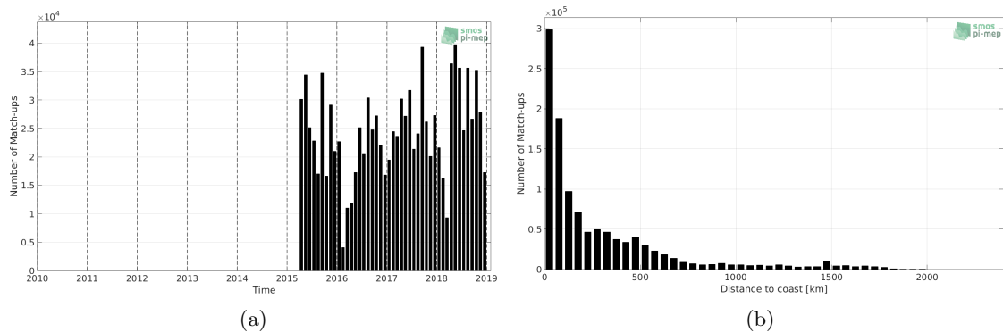
Figure 1: Number of match-ups between TSG-LEGOS-DM and SMAP-L3-JPL-V4.2-MONTHLY-60KM SSS as a function of time (a) and as function of the distance to coast (b) over the North Atlantic Ocean Pi-MEP region and for the full satellite product period.
