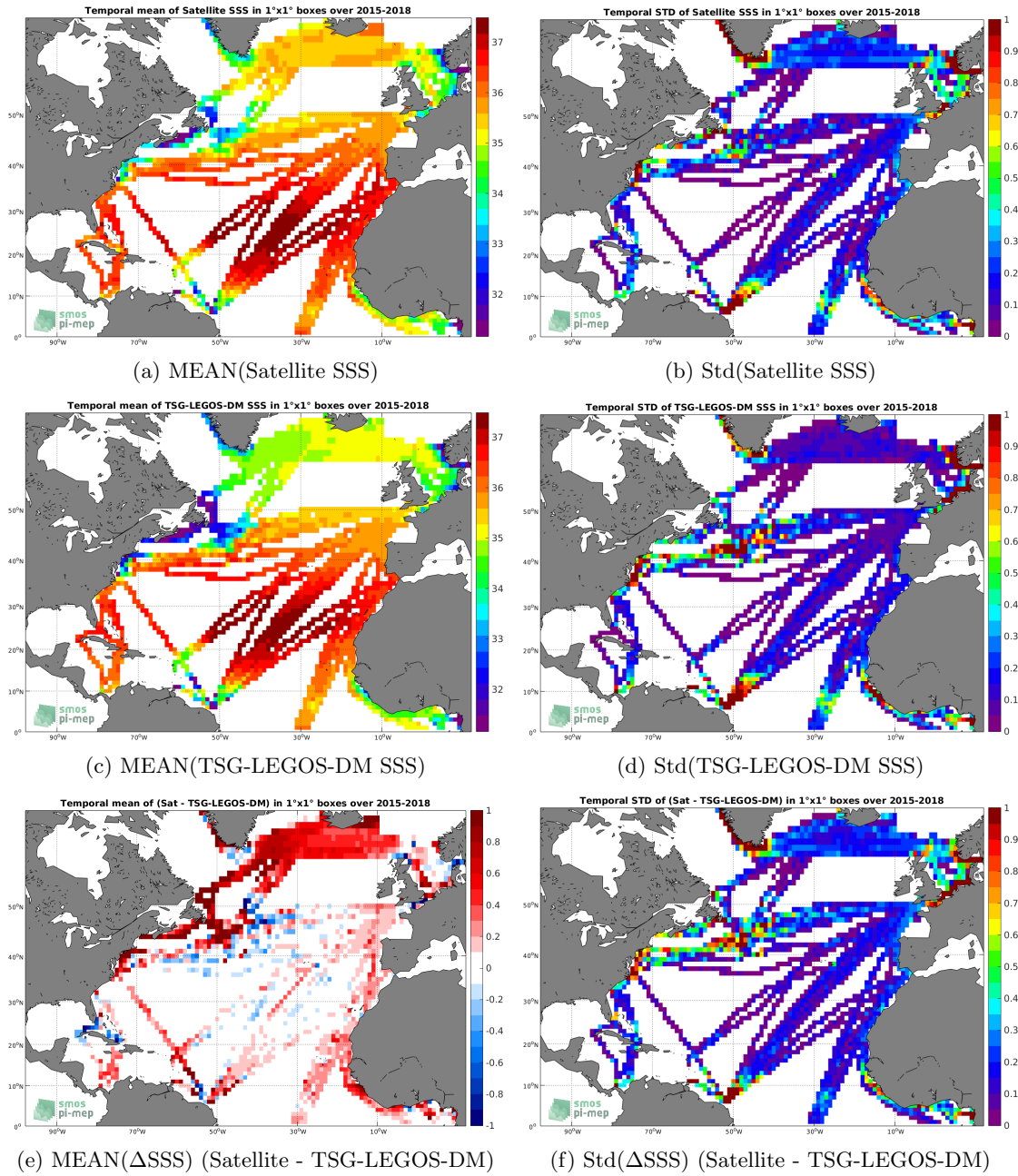
Figure 6: Temporal mean (left) and Std (right) of SSS from SMAP-L3-JPL-V4.2-MONTHLY-60KM (top), TSG-LEGOS-DM (middle), and of \Delta SSS (Satellite - TSG-LEGOS-DM). Only match-up pairs are used to generate these maps.
