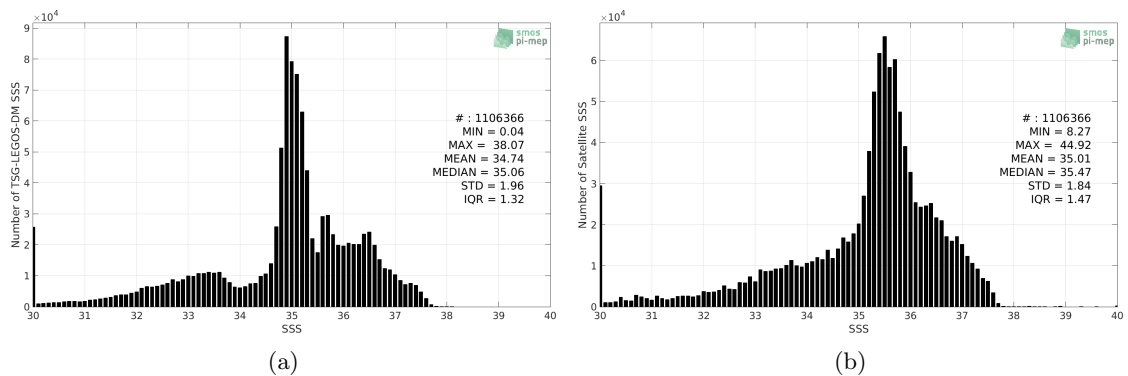
Figure 2: Histograms of SSS from TSG-LEGOS-DM (a) and SMAP-L3-JPL-V4.2-MONTHLY-60KM (b) considering all match-up pairs per bins of 0.1 over the North Atlantic Ocean Pi-MEP region and for the full satellite product period.
