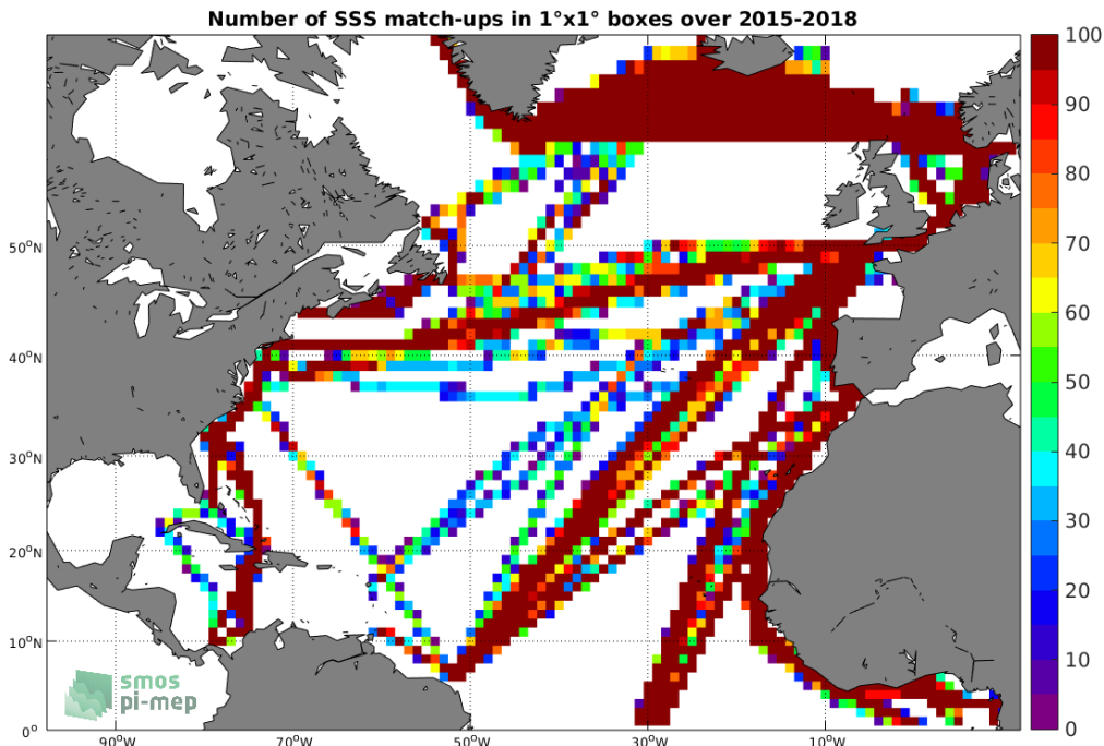
Figure 4: Number of SSS match-ups between TSG-LEGOS-DM SSS and the SMAP-L3-JPL-V4.2-MONTHLY-60KM SSS product for the North Atlantic Ocean Pi-MEP region over 1^\circ \times 1^\circ boxes and for the full satellite product period.
