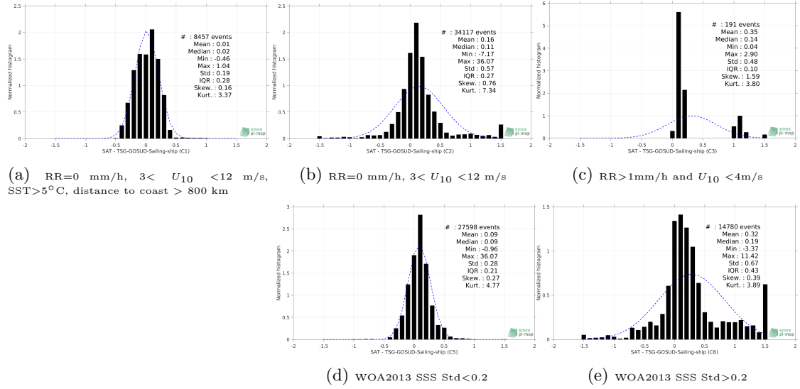
Figure 13: Normalized histogram of \Delta SSS (SMAP-L3-JPL-V4.2-MONTHLY-60KM - TSG-GOSUD-Sailing-ship) for 5 different subdatasets corresponding to: RR=0 mm/h, 3 < U_{10} < 12 m/s, SST > 5°C, distance to coast > 800 km (a), RR=0 mm/h, 3 < U_{10} < 12 m/s (b), RR > 1mm/h and U_{10} < 4 m/s (c), WOA2013 SSS Std < 0.2 (d), WOA2013 SSS Std > 0.2 (e).
