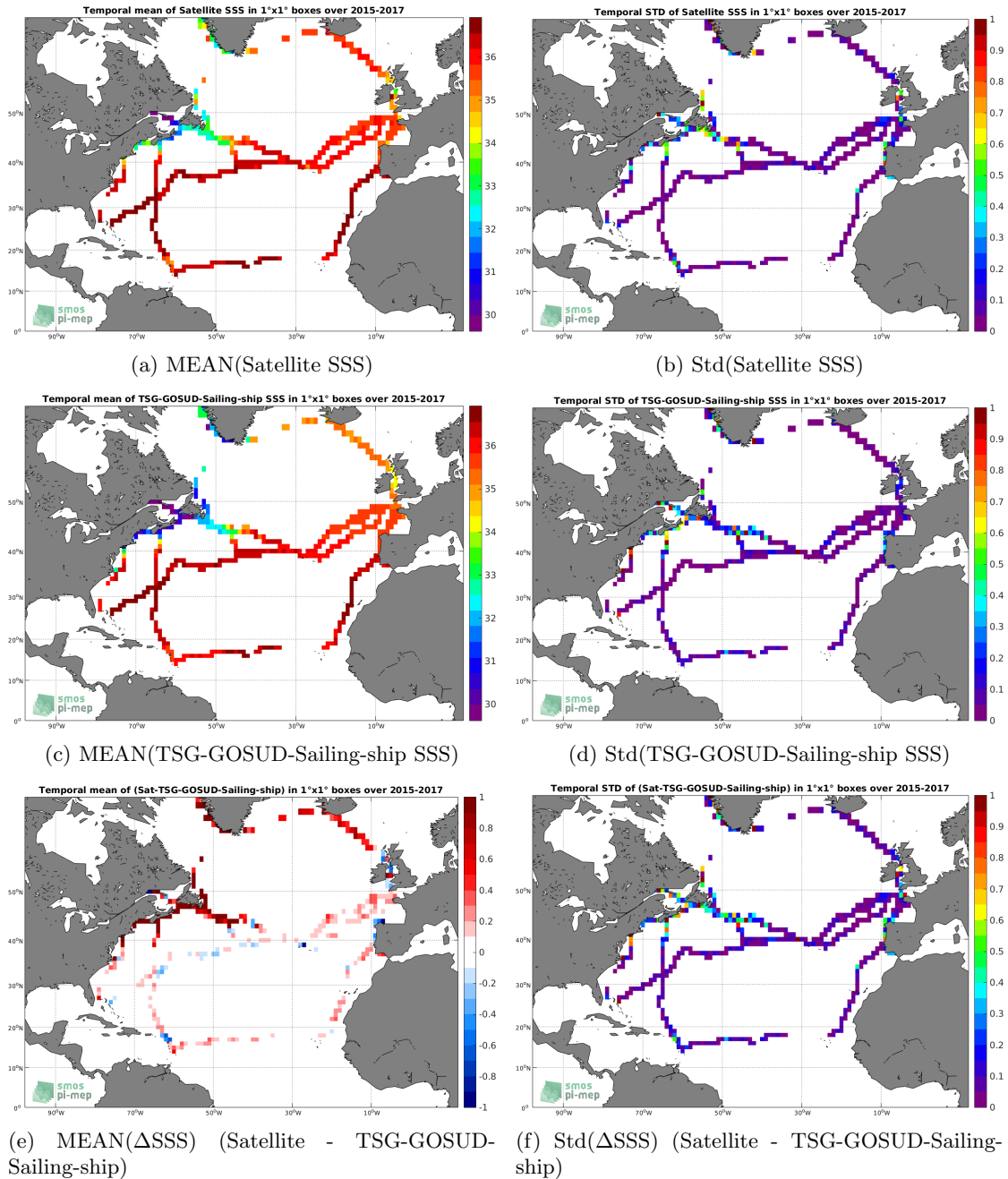
Figure 6: Temporal mean (left) and Std (right) of SSS from SMAP-L3-JPL-V4.2-MONTHLY-60KM (top), TSG-GOSUD-Sailing-ship (middle), and of \Delta SSS (Satellite - TSG-GOSUD-Sailing-ship). Only match-up pairs are used to generate these maps.
