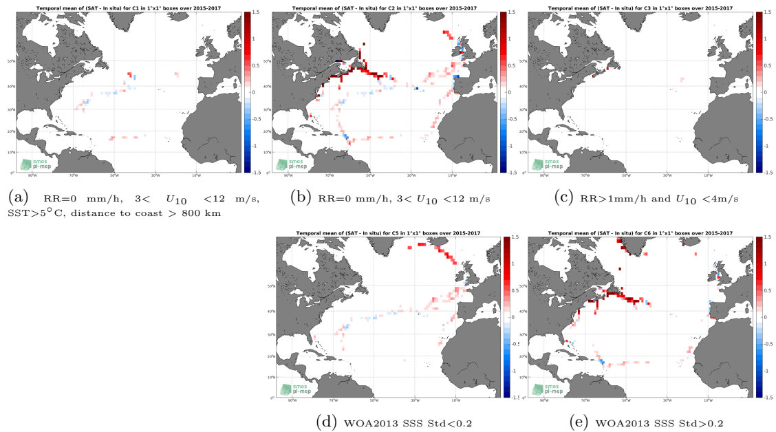
Figure 12: Temporal mean gridded over spatial boxes of size 1^\circ \times 1^\circ of \Delta SSS (SMAP-L3-JPL-V4.2-MONTHLY-60KM - TSG-GOSUD-Sailing-ship) for 5 different subdatasets corresponding to:RR=0 mm/h, 3 < U_{10} < 12 m/s, SST > 5^\circ\text{C} , distance to coast > 800 km (a), RR=0 mm/h, 3 < U_{10} < 12 m/s (b), RR > 1 mm/h and U_{10} < 4 m/s (c), WOA2013 SSS Std < 0.2 (d), WOA2013 SSS Std > 0.2 (e).
