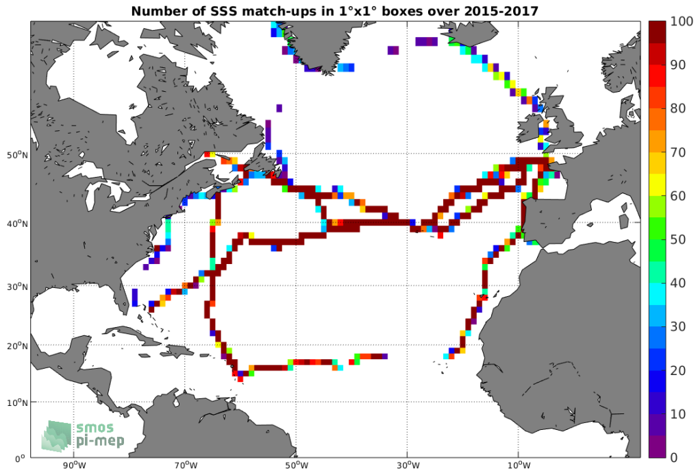
Figure 4: Number of SSS match-ups between TSG-GOSUD-Sailing-ship SSS and the SMAP-L3-JPL-V4.2-MONTHLY-60KM SSS product for the North Atlantic Ocean Pi-MEP region over 1^\circ \times 1^\circ boxes and for the full satellite product period.
