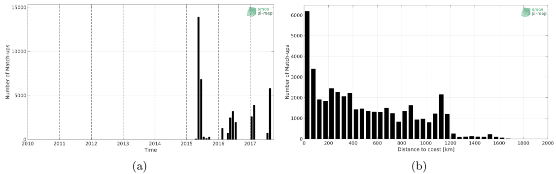
Figure 1: Number of match-ups between TSG-GOSUD-Sailing-ship and SMAP-L3-JPL-V4.2-MONTHLY-60KM SSS as a function of time (a) and as function of the distance to coast (b) over the North Atlantic Ocean Pi-MEP region and for the full satellite product period.
