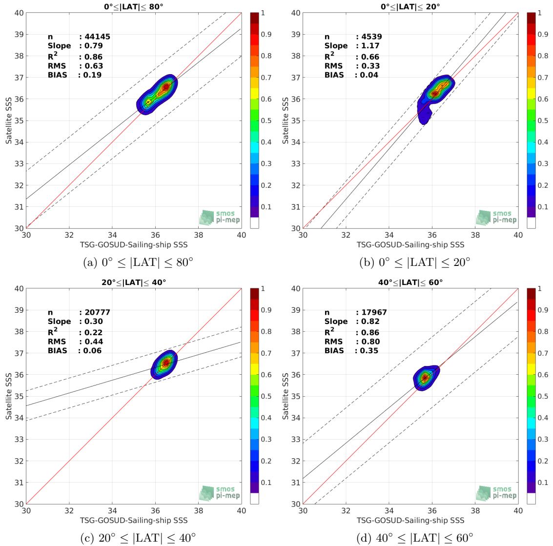
Figure 9: Contour maps of the concentration of SMAP-L3-JPL-V4.2-MONTHLY-60KM SSS (y-axis) versus TSG-GOSUD-Sailing-ship SSS (x-axis) at match-up pairs for different latitude bands. For each plot, the red line shows x=y . The black thin and dashed lines indicate a linear fit through the data cloud and the \pm 95\% confidence levels, respectively. The number match-up pairs n , the slope and R^2 coefficient of the linear fit, the root mean square (RMS) and the mean bias between satellite and in situ data are indicated for each latitude band in each plots.
