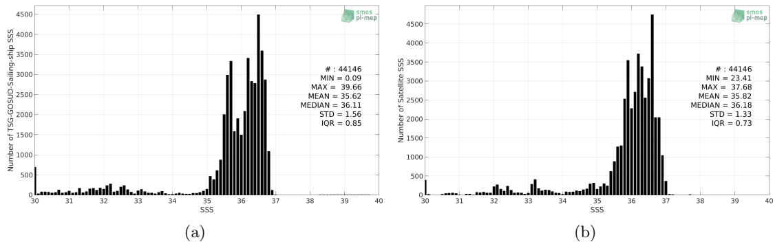
Figure 2: Histograms of SSS from TSG-GOSUD-Sailing-ship (a) and SMAP-L3-JPL-V4.2-MONTHLY-60KM (b) considering all match-up pairs per bins of 0.1 over the North Atlantic Ocean Pi-MEP region and for the full satellite product period.
