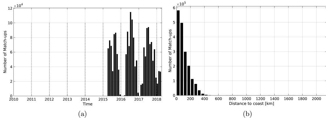
Figure 1: Number of match-ups between TSG-SAMOS and SMAP-L3-JPL-V4-8DAY-RUNNING-60KM SSS as a function of time (a) and as function of the distance to coast (b) over the North Atlantic Ocean Pi-MEP region and for the full satellite product period.
