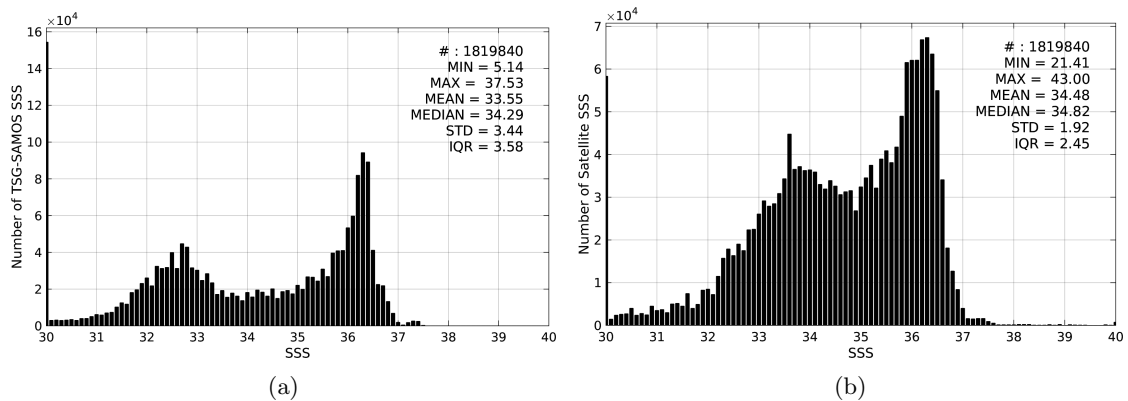
Figure 2: Histograms of SSS from TSG-SAMOS (a) and SMAP-L3-JPL-V4-8DAY-RUNNING-60KM (b) considering all match-up pairs per bins of 0.1 over the North Atlantic Ocean Pi-MEP region and for the full satellite product period.
