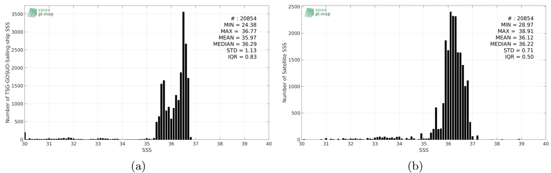
Figure 2: Histograms of SSS from TSG-GOSUD-Sailing-ship (a) and SMAP-L3-JPL-V4-8DAY-RUNNING-60KM (b) considering all match-up pairs per bins of 0.1 over the North Atlantic Ocean Pi-MEP region and for the full satellite product period.
