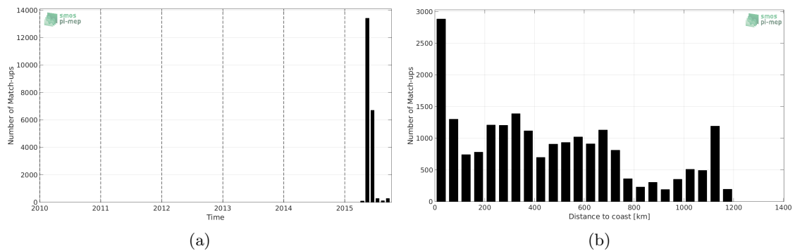
Figure 1: Number of match-ups between TSG-GOSUD-Sailing-ship and SMAP-L3-JPL-V4-8DAY-RUNNING-60KM SSS as a function of time (a) and as function of the distance to coast (b) over the North Atlantic Ocean Pi-MEP region and for the full satellite product period.
