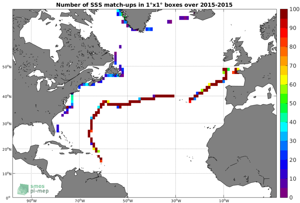
Figure 4: Number of SSS match-ups between TSG-GOSUD-Sailing-ship SSS and the SMAP-L3-JPL-V4-8DAY-RUNNING-60KM SSS product for the North Atlantic Ocean Pi-MEP region over 1^\circ \times 1^\circ boxes and for the full satellite product period.
