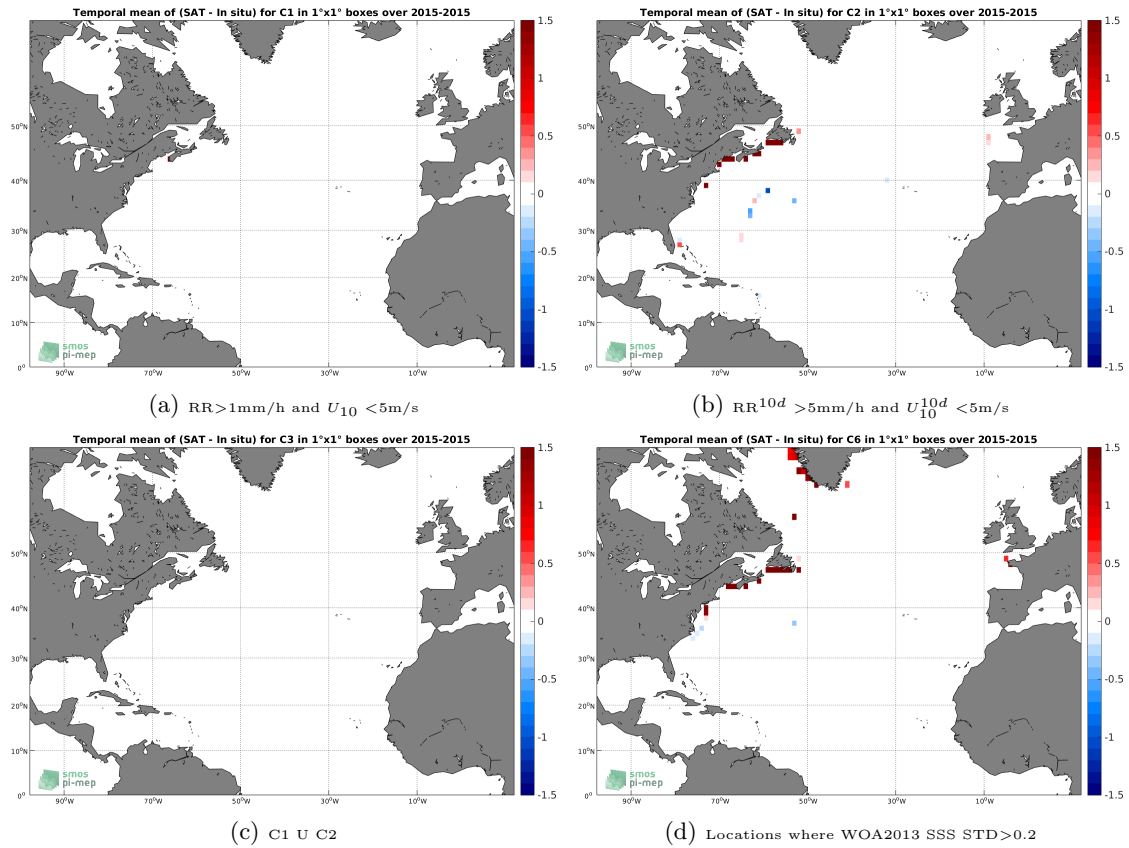
Figure 12: Temporal mean gridded over spatial boxes of size 1^\circ \times 1^\circ of \Delta SSS (SMAP-L3-JPL-V4-8DAY-RUNNING-60KM - TSG-GOSUD-Sailing-ship) for 4 different subdatasets corresponding to: RR > 1\text{mm/h} and U_{10} < 5\text{m/s} (a), RR^{10d} > 5\text{mm/h} and U_{10}^{10d} < 5\text{m/s} (b), C1 U C2 (c), Locations where WOA2013 SSS STD > 0.2 (d).
