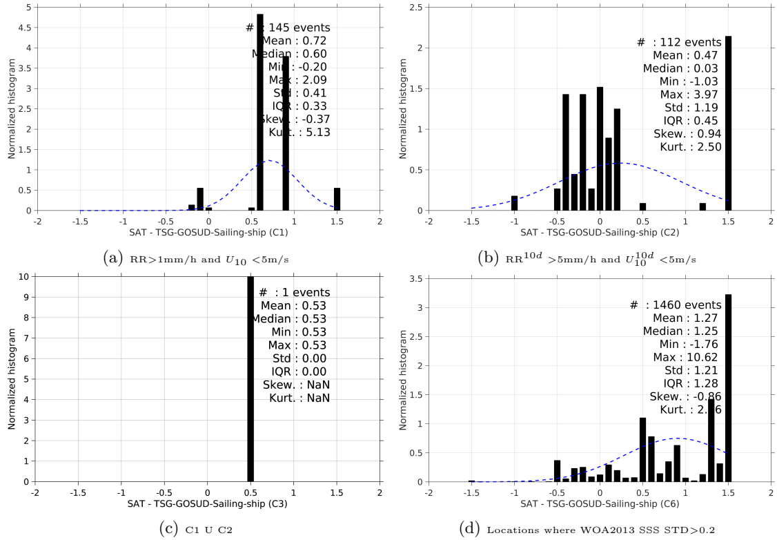
Figure 13: Normalized histogram of \Delta\text{SSS} (SMAP-L3-JPL-V4-8DAY-RUNNING-60KM - TSG-GOSUD-Sailing-ship) for 6 different subdatasets corresponding to: RR > 1mm/h and U_{10} < 5\text{m/s} (a), RR^{10d} > 5\text{mm/h} and U_{10}^{10d} < 5\text{m/s} (b), C1 U C2 (c), Locations where WOA2013 SSS STD > 0.2 (d).
