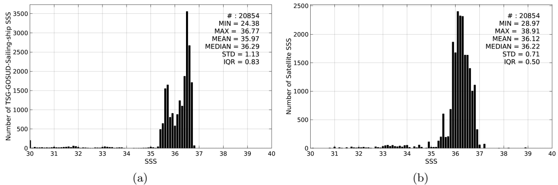
Figure 2: Histograms of SSS from TSG-GOSUD-Sailing-ship (a) and SMAP-L3-JPL-V4-8DAY-RUNNING-60KM (b) considering all match-up pairs per bins of 0.1 over the North Atlantic Ocean Pi-MEP region and for the full satellite product period.
