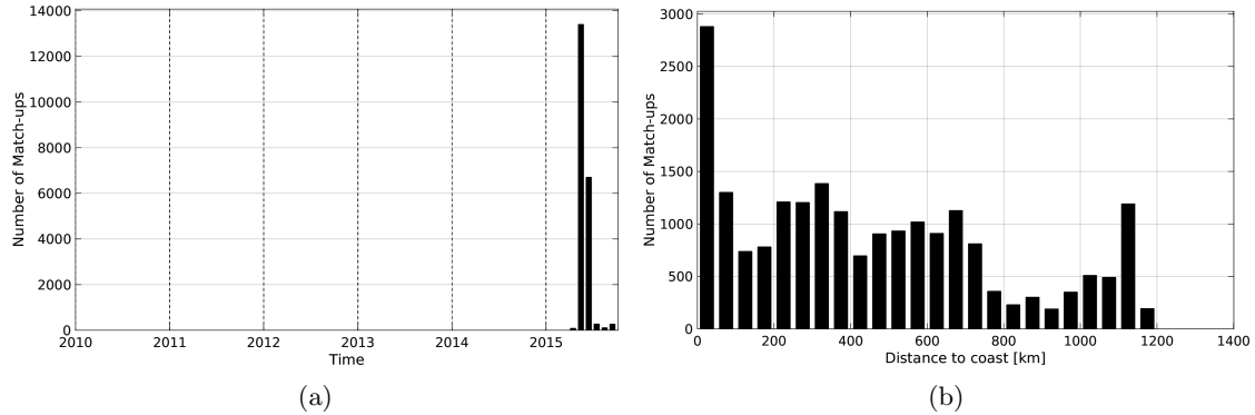
Figure 1: Number of match-ups between TSG-GOSUD-Sailing-ship and SMAP-L3-JPL-V4-8DAY-RUNNING-60KM SSS as a function of time (a) and as function of the distance to coast (b) over the North Atlantic Ocean Pi-MEP region and for the full satellite product period.
