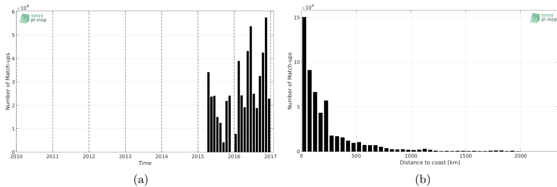
Figure 1: Number of match-ups between TSG-GOSUD-Research-vessel and SMAP-L3-JPL-V4-8DAY-RUNNING-60KM SSS as a function of time (a) and as function of the distance to coast (b) over the North Atlantic Ocean Pi-MEP region and for the full satellite product period.
