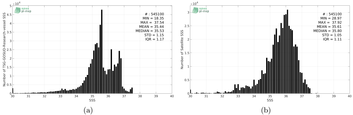
Figure 2: Histograms of SSS from TSG-GOSUD-Research-vessel (a) and SMAP-L3-JPL-V4-8DAY-RUNNING-60KM (b) considering all match-up pairs per bins of 0.1 over the North Atlantic Ocean Pi-MEP region and for the full satellite product period.
