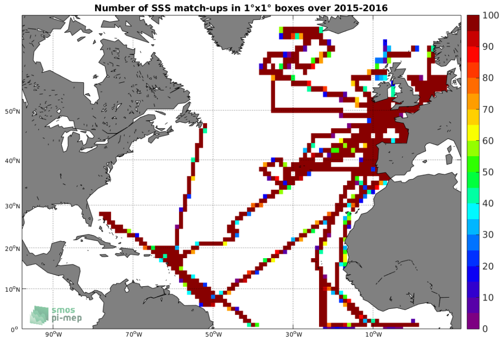
Figure 4: Number of SSS match-ups between TSG-GOSUD-Research-vessel SSS and the SMAP-L3-JPL-V4-8DAY-RUNNING-60KM SSS product for the North Atlantic Ocean Pi-MEP region over 1°x1° boxes and for the full satellite product period.
