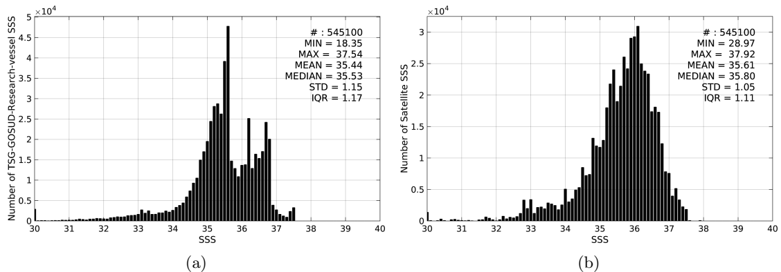
Figure 2: Histograms of SSS from TSG-GOSUD-Research-vessel (a) and SMAP-L3-JPL-V4-8DAY-RUNNING-60KM (b) considering all match-up pairs per bins of 0.1 over the North Atlantic Ocean Pi-MEP region and for the full satellite product period.
