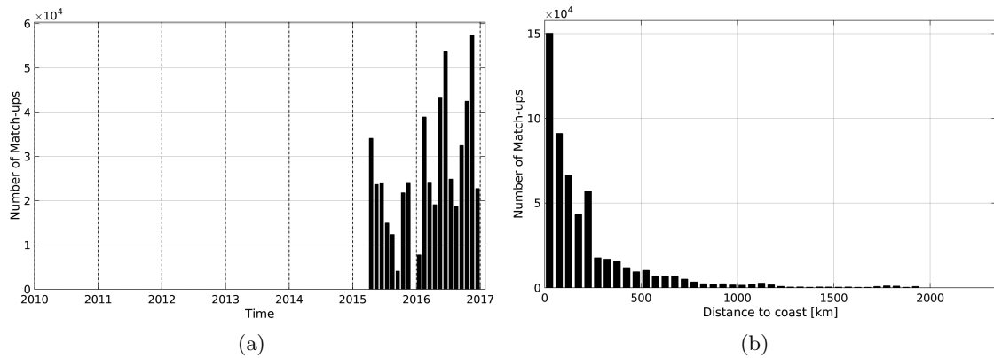
Figure 1: Number of match-ups between TSG-GOSUD-Research-vessel and SMAP-L3-JPL-V4-8DAY-RUNNING-60KM SSS as a function of time (a) and as function of the distance to coast (b) over the North Atlantic Ocean Pi-MEP region and for the full satellite product period.
