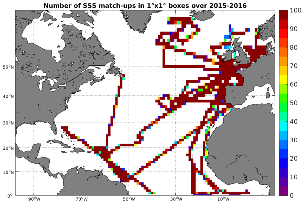
Figure 4: Number of SSS match-ups between TSG-GOSUD-Research-vessel SSS and the SMAP-L3-JPL-V4-8DAY-RUNNING-60KM SSS product for the North Atlantic Ocean Pi-MEP region over 1^\circ \times 1^\circ boxes and for the full satellite product period.
