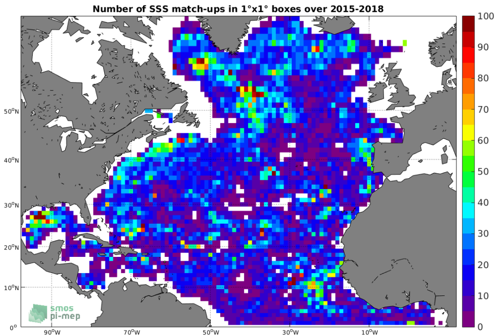
Figure 4: Number of SSS match-ups between Argo SSS and the SMAP-L3-JPL-V4-8DAY-RUNNING-60KM SSS product for the North Atlantic Ocean Pi-MEP region over 1^\circ \times 1^\circ boxes and for the full satellite product period.
