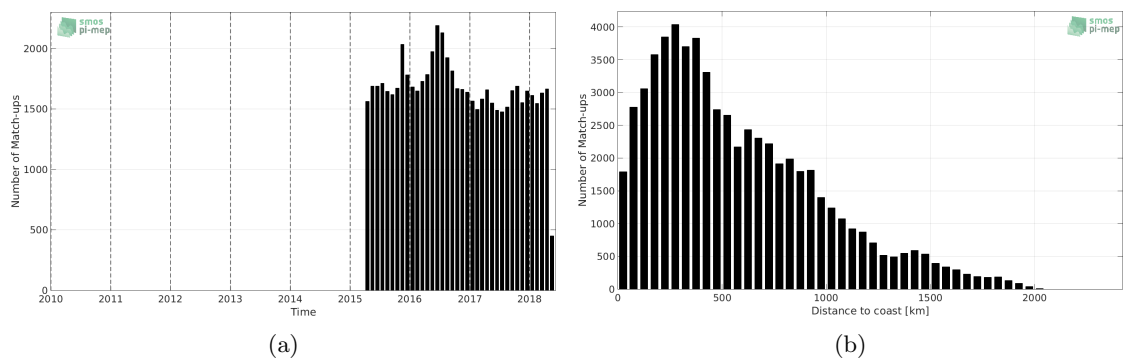
Figure 1: Number of match-ups between Argo and SMAP-L3-JPL-V4-8DAY-RUNNING-60KM SSS as a function of time (a) and as function of the distance to coast (b) over the North Atlantic Ocean Pi-MEP region and for the full satellite product period.
