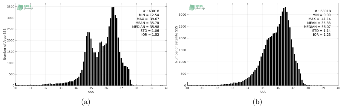
Figure 2: Histograms of SSS from Argo (a) and SMAP-L3-JPL-V4-8DAY-RUNNING-60KM (b) considering all match-up pairs per bins of 0.1 over the North Atlantic Ocean Pi-MEP region and for the full satellite product period.
