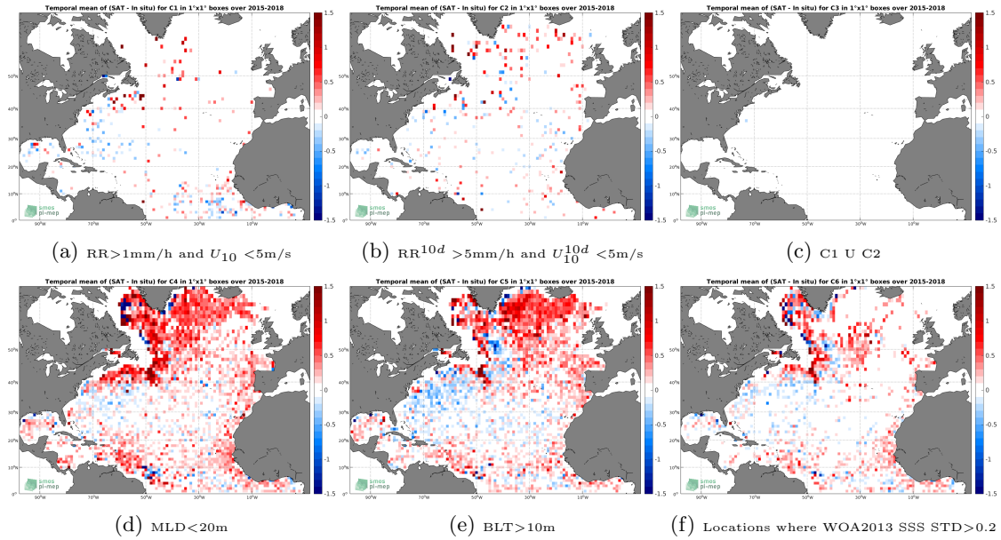
Figure 12: Temporal mean gridded over spatial boxes of size 1^\circ \times 1^\circ of \Delta SSS (SMAP-L3-JPL-V4-8DAY-RUNNING-60KM - Argo) for 6 different subdatasets corresponding to: RR > 1\text{mm/h} and U_{10} < 5\text{m/s} (a), RR^{10d} > 5\text{mm/h} and U_{10}^{10d} < 5\text{m/s} (b), C1 U C2 (c), MLD < 20\text{m} (d), BLT > 10\text{m} (e), Locations where WOA2013 SSS STD > 0.2 (f).
