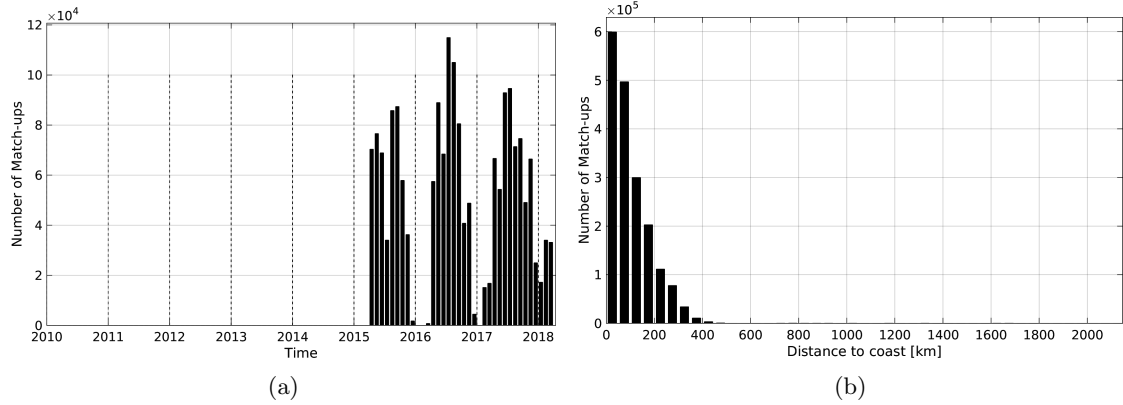
Figure 1: Number of match-ups between TSG-SAMOS and SMAP-L3-JPL-V4-MONTHLY-60KM SSS as a function of time (a) and as function of the distance to coast (b) over the North Atlantic Ocean Pi-MEP region and for the full satellite product period.
