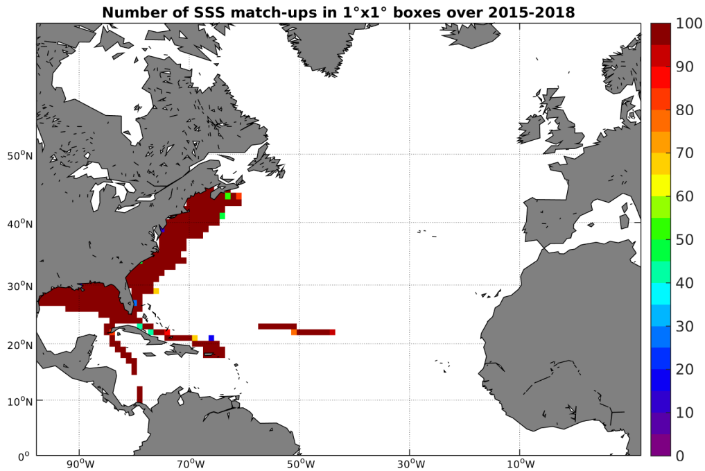
Figure 4: Number of SSS match-ups between TSG-SAMOS SSS and the SMAP-L3-JPL-V4-MONTHLY-60KM SSS product for the North Atlantic Ocean Pi-MEP region over 1^\circ \times 1^\circ boxes and for the full satellite product period.
