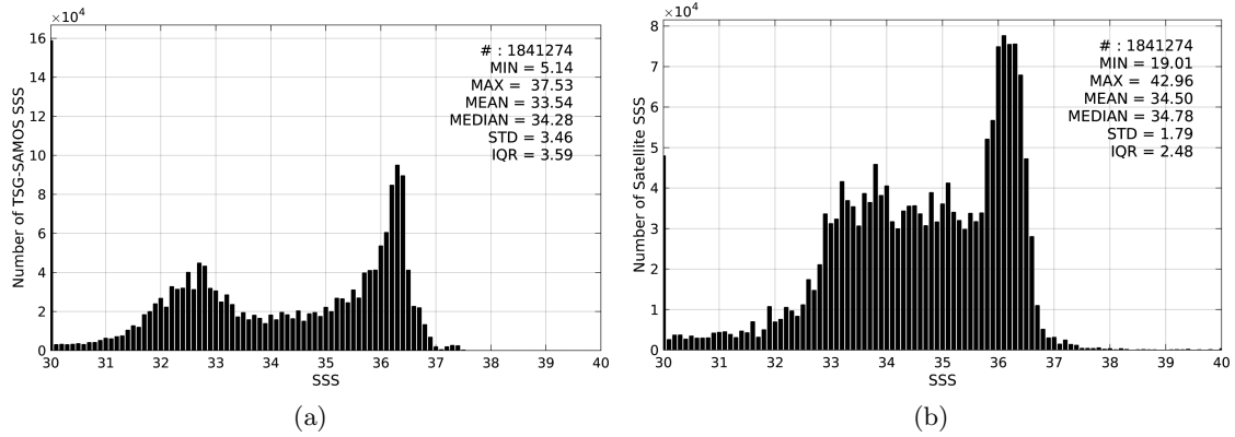
Figure 2: Histograms of SSS from TSG-SAMOS (a) and SMAP-L3-JPL-V4-MONTHLY-60KM (b) considering all match-up pairs per bins of 0.1 over the North Atlantic Ocean Pi-MEP region and for the full satellite product period.
