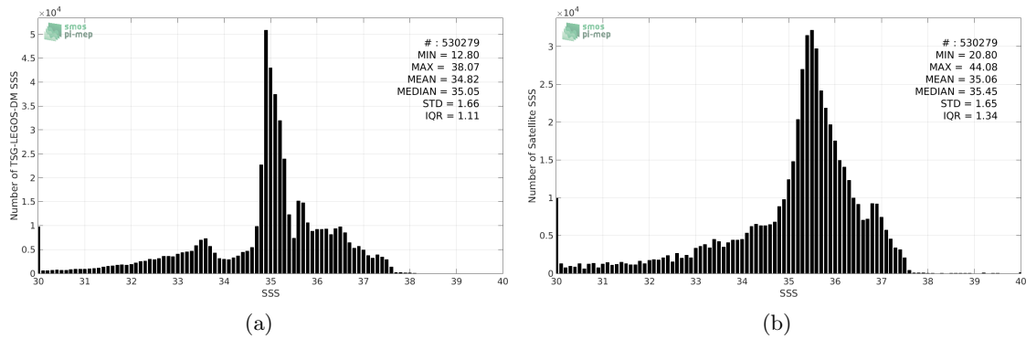
Figure 2: Histograms of SSS from TSG-LEGOS-DM (a) and SMAP-L3-JPL-V4-MONTHLY-60KM (b) considering all match-up pairs per bins of 0.1 over the North Atlantic Ocean Pi-MEP region and for the full satellite product period.
