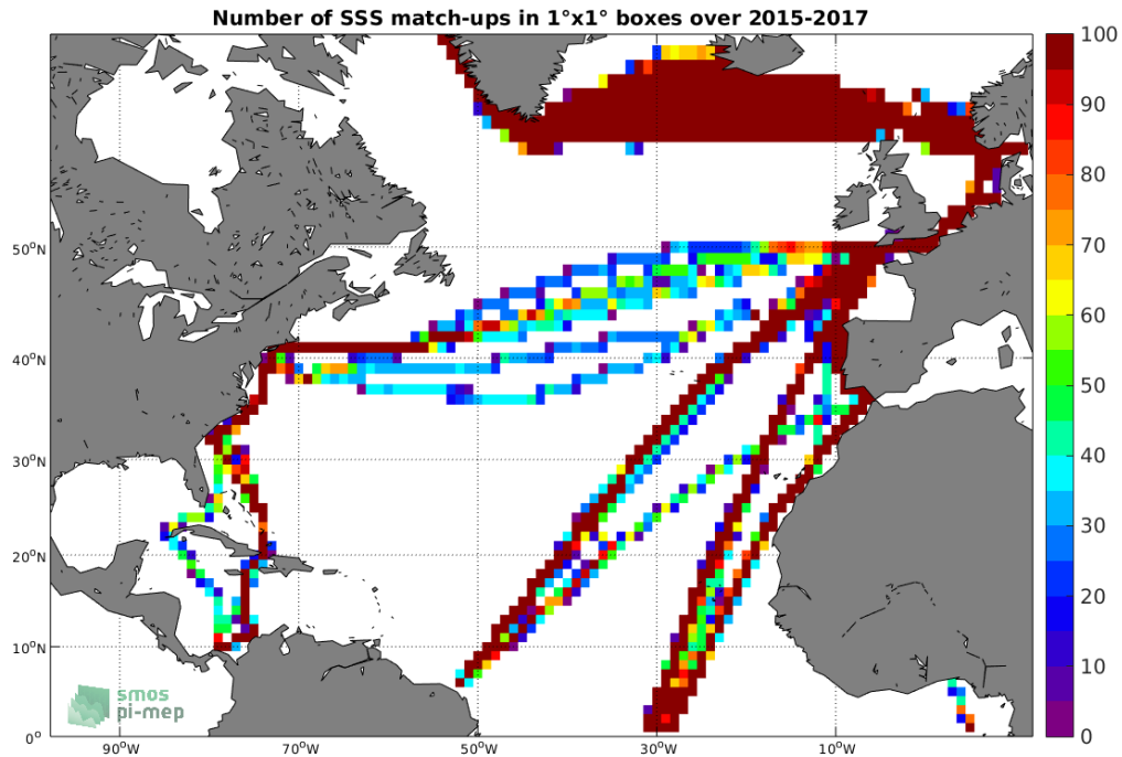
Figure 4: Number of SSS match-ups between TSG-LEGOS-DM SSS and the SMAP-L3-JPL-V4-MONTHLY-60KM SSS product for the North Atlantic Ocean Pi-MEP region over 1^\circ \times 1^\circ boxes and for the full satellite product period.
