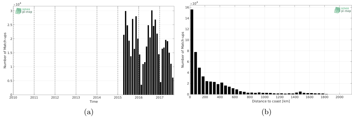
Figure 1: Number of match-ups between TSG-LEGOS-DM and SMAP-L3-JPL-V4-MONTHLY-60KM SSS as a function of time (a) and as function of the distance to coast (b) over the North Atlantic Ocean Pi-MEP region and for the full satellite product period.
