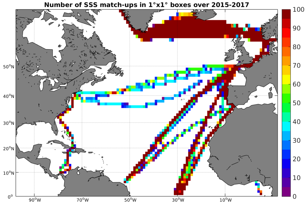
Figure 4: Number of SSS match-ups between TSG-LEGOS-DM SSS and the SMAP-L3-JPL-V4-MONTHLY-60KM SSS product for the North Atlantic Ocean Pi-MEP region over 1°x1° boxes and for the full satellite product period.
