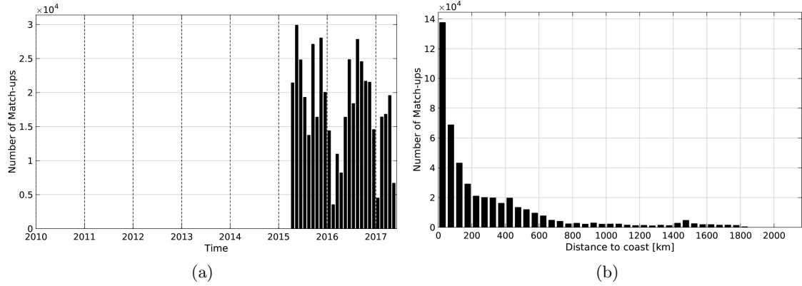
Figure 1: Number of match-ups between TSG-LEGOS-DM and SMAP-L3-JPL-V4-MONTHLY-60KM SSS as a function of time (a) and as function of the distance to coast (b) over the North Atlantic Ocean Pi-MEP region and for the full satellite product period.
