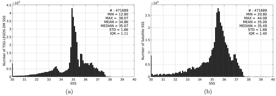
Figure 2: Histograms of SSS from TSG-LEGOS-DM (a) and SMAP-L3-JPL-V4-MONTHLY-60KM (b) considering all match-up pairs per bins of 0.1 over the North Atlantic Ocean Pi-MEP region and for the full satellite product period.
