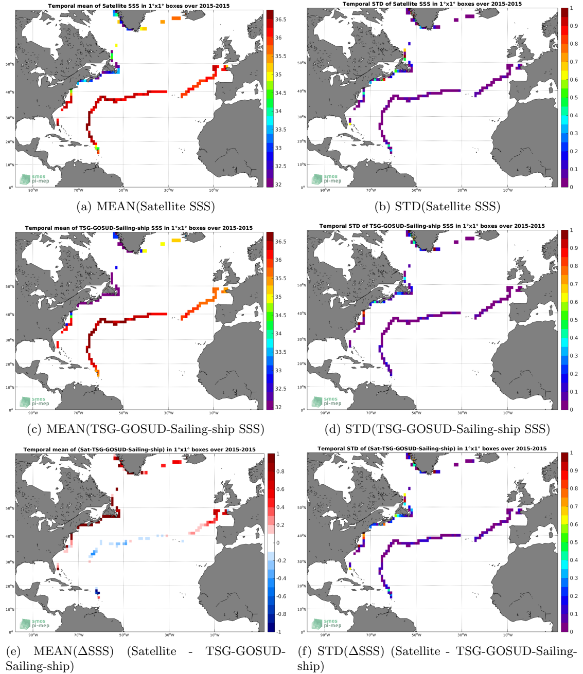
Figure 6: Temporal mean (left) and STD (right) of SSS from SMAP-L3-JPL-V4-MONTHLY-60KM (top), TSG-GOSUD-Sailing-ship (middle), and of \Delta SSS (Satellite - TSG-GOSUD-Sailing-ship). Only match-up pairs are used to generate these maps.
