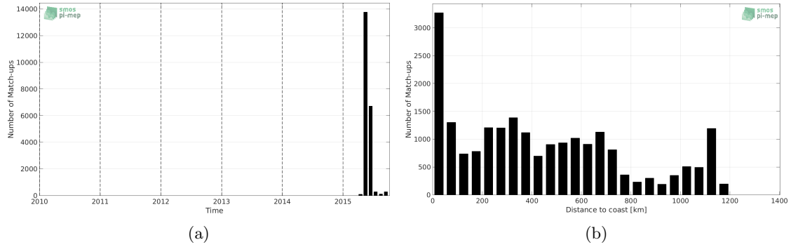
Figure 1: Number of match-ups between TSG-GOSUD-Sailing-ship and SMAP-L3-JPL-V4-MONTHLY-60KM SSS as a function of time (a) and as function of the distance to coast (b) over the North Atlantic Ocean Pi-MEP region and for the full satellite product period.
