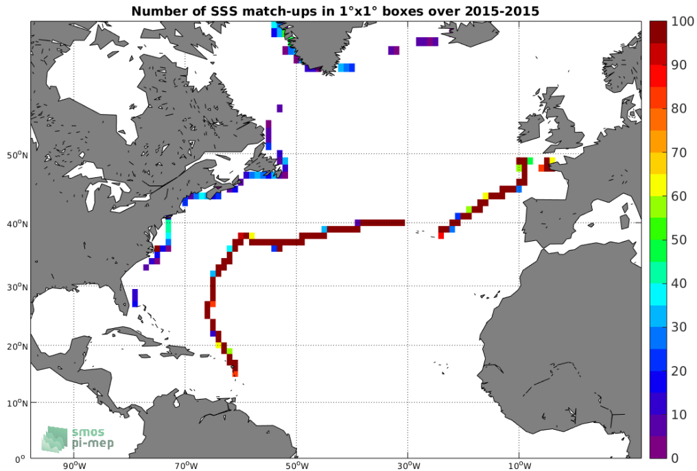
Figure 4: Number of SSS match-ups between TSG-GOSUD-Sailing-ship SSS and the SMAP-L3-JPL-V4-MONTHLY-60KM SSS product for the North Atlantic Ocean Pi-MEP region over 1^\circ \times 1^\circ boxes and for the full satellite product period.
