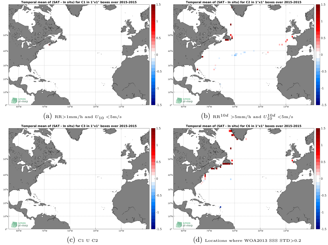
Figure 12: Temporal mean gridded over spatial boxes of size 1^\circ \times 1^\circ of \Delta SSS (SMAP-L3-JPL-V4-MONTHLY-60KM - TSG-GOSUD-Sailing-ship) for 4 different subdatasets corresponding to: RR > 1\text{mm/h} and U_{10} < 5\text{m/s} (a), RR^{10d} > 5\text{mm/h} and U_{10}^{10d} < 5\text{m/s} (b), C1 U C2 (c), Locations where WOA2013 SSS STD > 0.2 (d).
