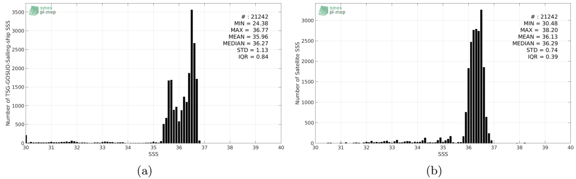
Figure 2: Histograms of SSS from TSG-GOSUD-Sailing-ship (a) and SMAP-L3-JPL-V4-MONTHLY-60KM (b) considering all match-up pairs per bins of 0.1 over the North Atlantic Ocean Pi-MEP region and for the full satellite product period.
