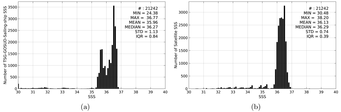
Figure 2: Histograms of SSS from TSG-GOSUD-Sailing-ship (a) and SMAP-L3-JPL-V4-MONTHLY-60KM (b) considering all match-up pairs per bins of 0.1 over the North Atlantic Ocean Pi-MEP region and for the full satellite product period.
