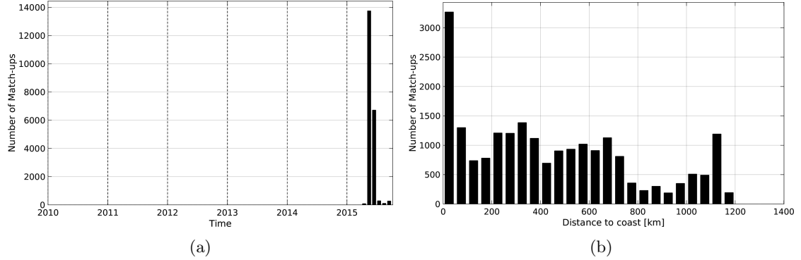
Figure 1: Number of match-ups between TSG-GOSUD-Sailing-ship and SMAP-L3-JPL-V4-MONTHLY-60KM SSS as a function of time (a) and as function of the distance to coast (b) over the North Atlantic Ocean Pi-MEP region and for the full satellite product period.
