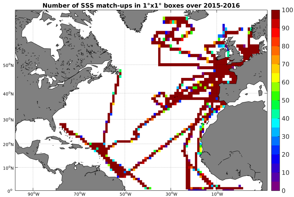
Figure 4: Number of SSS match-ups between TSG-GOSUD-Research-vessel SSS and the SMAP-L3-JPL-V4-MONTHLY-60KM SSS product for the North Atlantic Ocean Pi-MEP region over 1^\circ \times 1^\circ boxes and for the full satellite product period.
