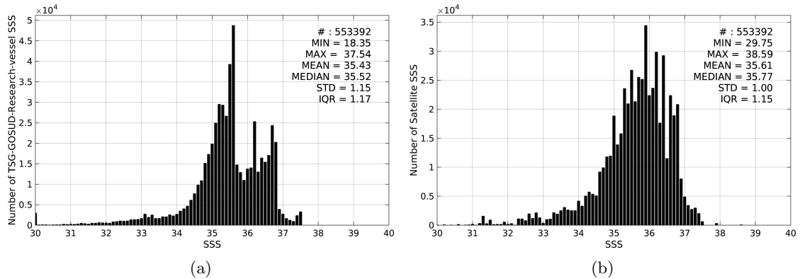
Figure 2: Histograms of SSS from TSG-GOSUD-Research-vessel (a) and SMAP-L3-JPL-V4-MONTHLY-60KM (b) considering all match-up pairs per bins of 0.1 over the North Atlantic Ocean Pi-MEP region and for the full satellite product period.
