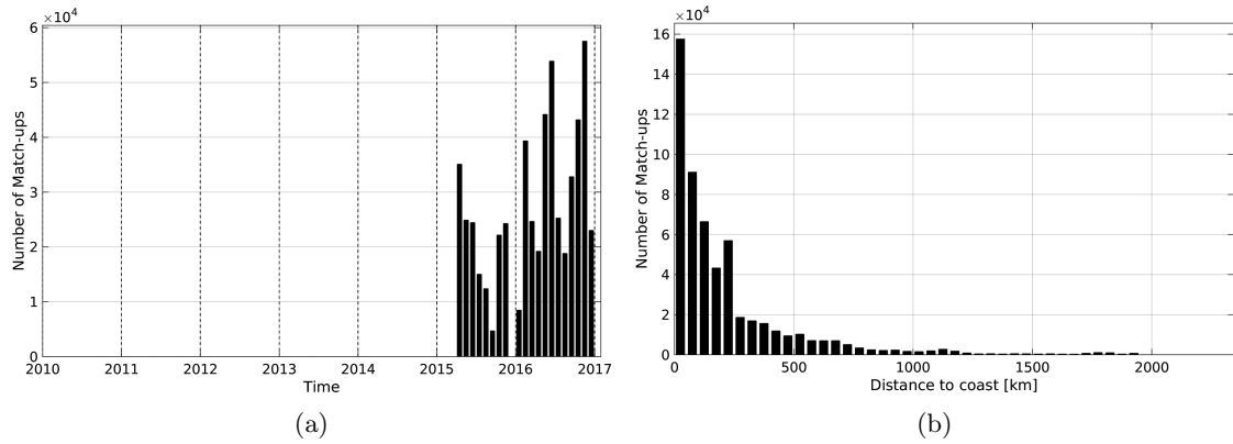
Figure 1: Number of match-ups between TSG-GOSUD-Research-vessel and SMAP-L3-JPL-V4-MONTHLY-60KM SSS as a function of time (a) and as function of the distance to coast (b) over the North Atlantic Ocean Pi-MEP region and for the full satellite product period.
