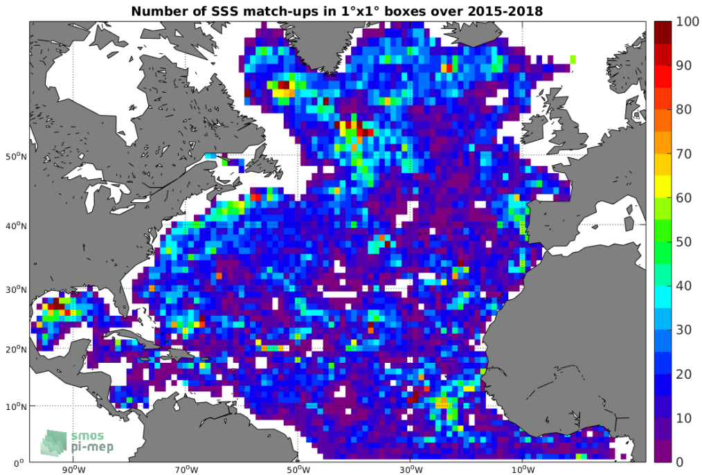
Figure 4: Number of SSS match-ups between Argo SSS and the SMAP-L3-JPL-V4-MONTHLY-60KM SSS product for the North Atlantic Ocean Pi-MEP region over 1^\circ \times 1^\circ boxes and for the full satellite product period.
