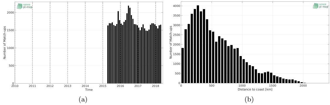
Figure 1: Number of match-ups between Argo and SMAP-L3-JPL-V4-MONTHLY-60KM SSS as a function of time (a) and as function of the distance to coast (b) over the North Atlantic Ocean Pi-MEP region and for the full satellite product period.
