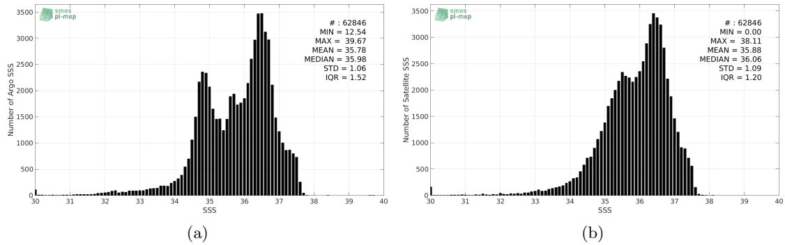
Figure 2: Histograms of SSS from Argo (a) and SMAP-L3-JPL-V4-MONTHLY-60KM (b) considering all match-up pairs per bins of 0.1 over the North Atlantic Ocean Pi-MEP region and for the full satellite product period.
