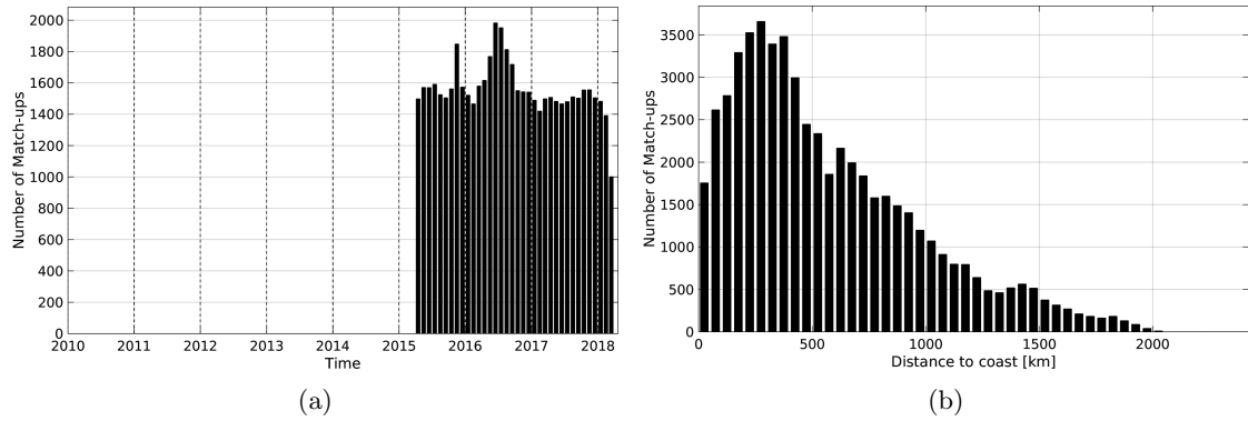
Figure 1: Number of match-ups between Argo and SMAP-L3-JPL-V4-MONTHLY-60KM SSS as a function of time (a) and as function of the distance to coast (b) over the North Atlantic Ocean Pi-MEP region and for the full satellite product period.
