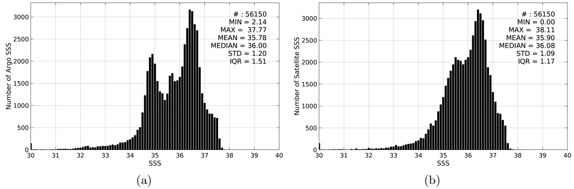
Figure 2: Histograms of SSS from Argo (a) and SMAP-L3-JPL-V4-MONTHLY-60KM (b) considering all match-up pairs per bins of 0.1 over the North Atlantic Ocean Pi-MEP region and for the full satellite product period.
