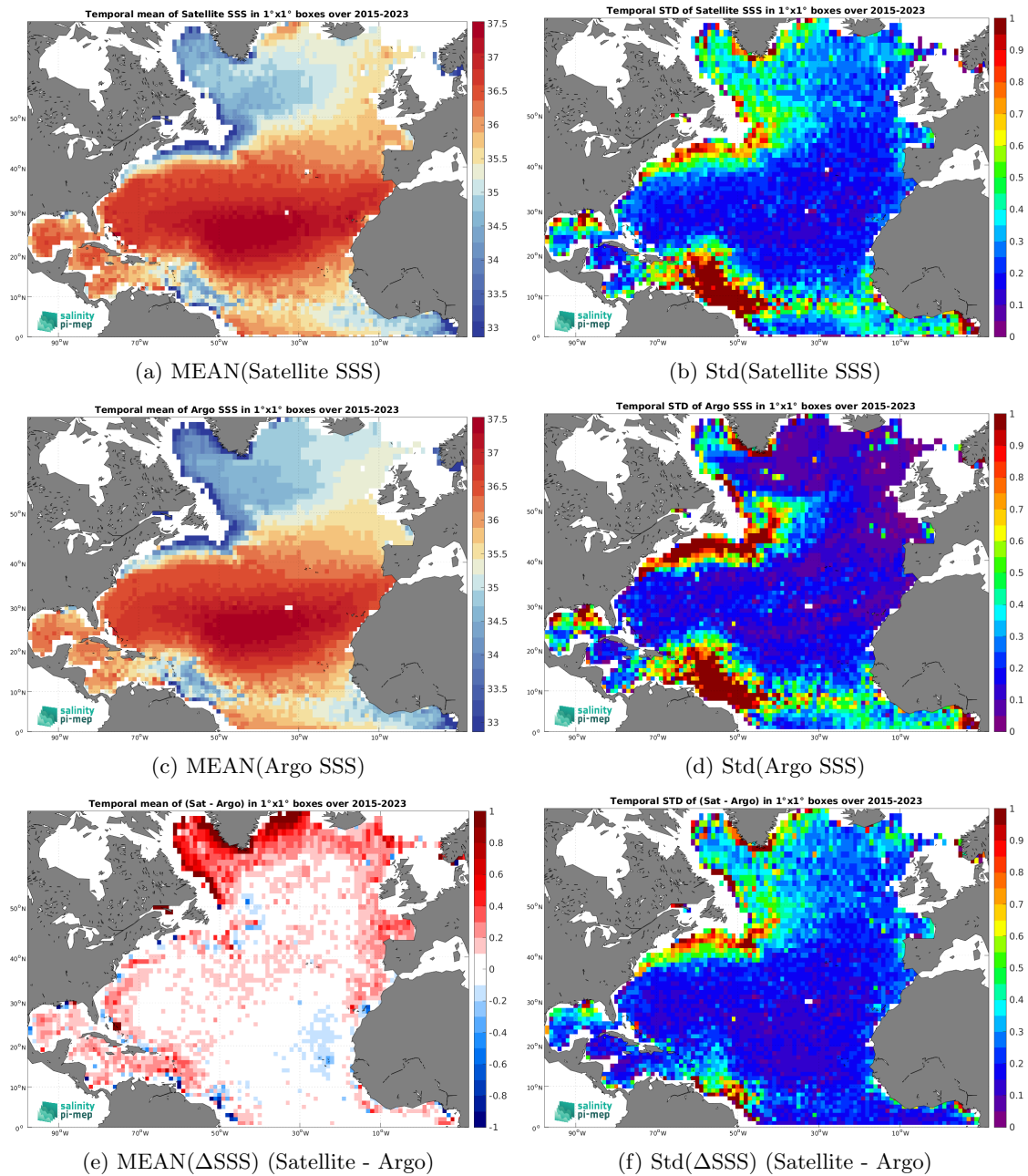
Figure 6: Temporal mean (left) and Std (right) of SSS from SMAP SSS L2-AVERAGED v5 (RSS) (top), Argo (middle), and of \Delta SSS (Satellite - Argo). Only match-up pairs are used to generate these maps.
