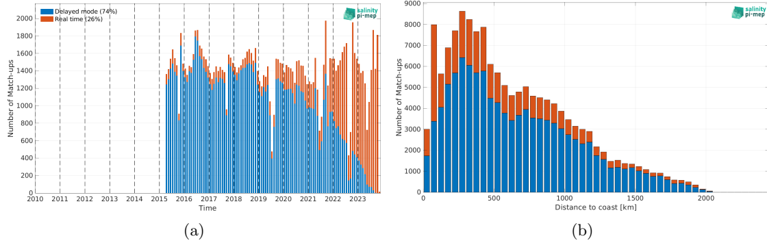
Figure 1: Number of match-ups between Argo and SMAP SSS L2-AVERAGED v5 (RSS) SSS as a function of time (a) and as function of the distance to coast (b) over the North Atlantic Ocean Pi-MEP region and for the full satellite product period.
