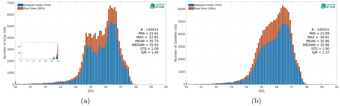
Figure 2: Histograms of SSS from Argo (a) and SMAP SSS L2-AVERAGED v5 (RSS) (b) considering all match-up pairs per bins of 0.1 over the North Atlantic Ocean Pi-MEP region and for the full satellite product period.
