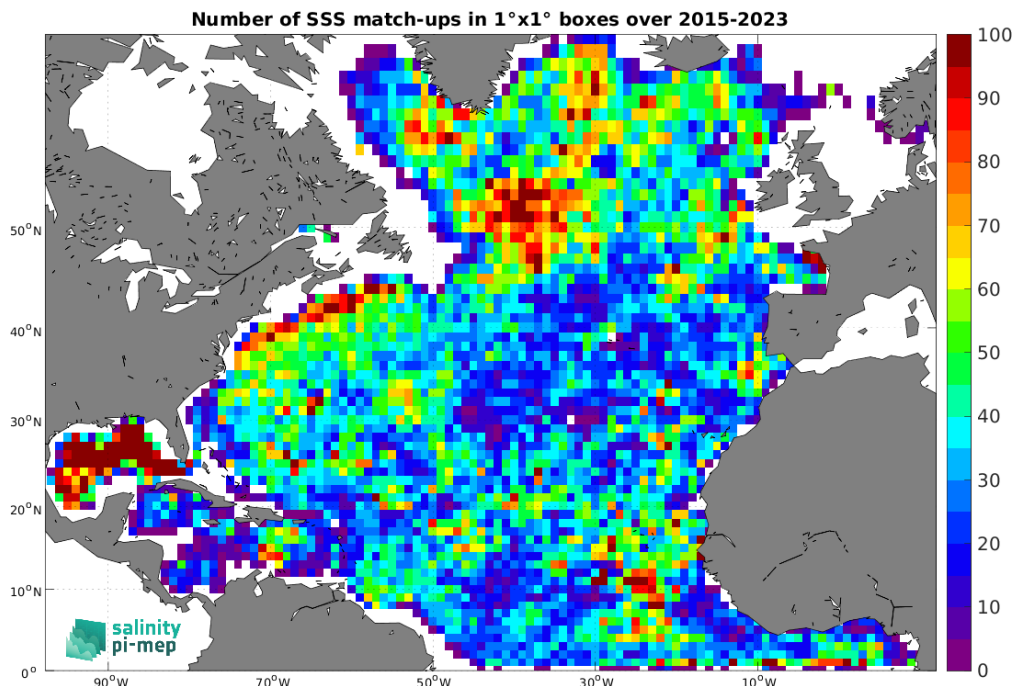
Figure 4: Number of SSS match-ups between Argo SSS and the SMAP SSS L2-AVERAGED v5 (RSS) SSS product for the North Atlantic Ocean Pi-MEP region over 1^\circ \times 1^\circ boxes and for the full satellite product period.
