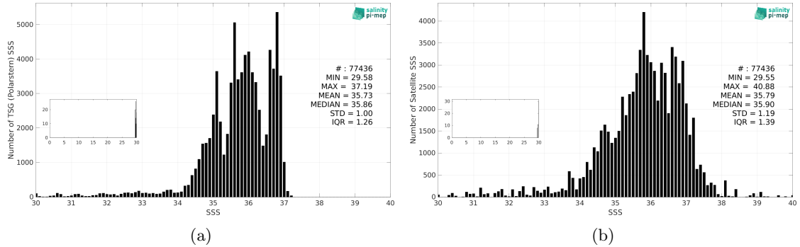
Figure 3: Histograms of SSS from TSG (Polarstern) (a) and SMAP SSS L2 v6 (RSS) (b) considering all match-up pairs per bins of 0.1 over the North Atlantic Ocean Pi-MEP region and for the full satellite product period.
