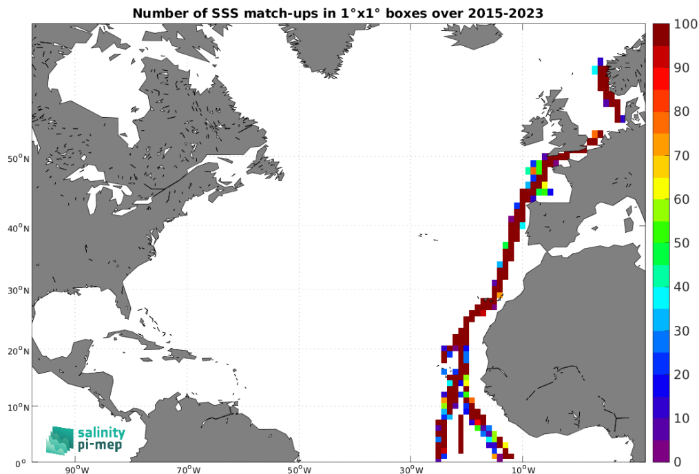
Figure 5: Number of SSS match-ups between TSG (Polarstern) SSS and the SMAP SSS L2 v6 (RSS) SSS product for the North Atlantic Ocean Pi-MEP region over 1^\circ \times 1^\circ boxes and for the full satellite product period.
