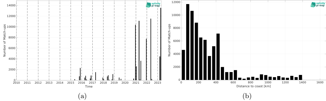
Figure 2: Number of match-ups between TSG (Polarstern) and SMAP SSS L2 v6 (RSS) SSS as a function of time (a) and as function of the distance to coast (b) over the North Atlantic Ocean Pi-MEP region and for the full satellite product period.
