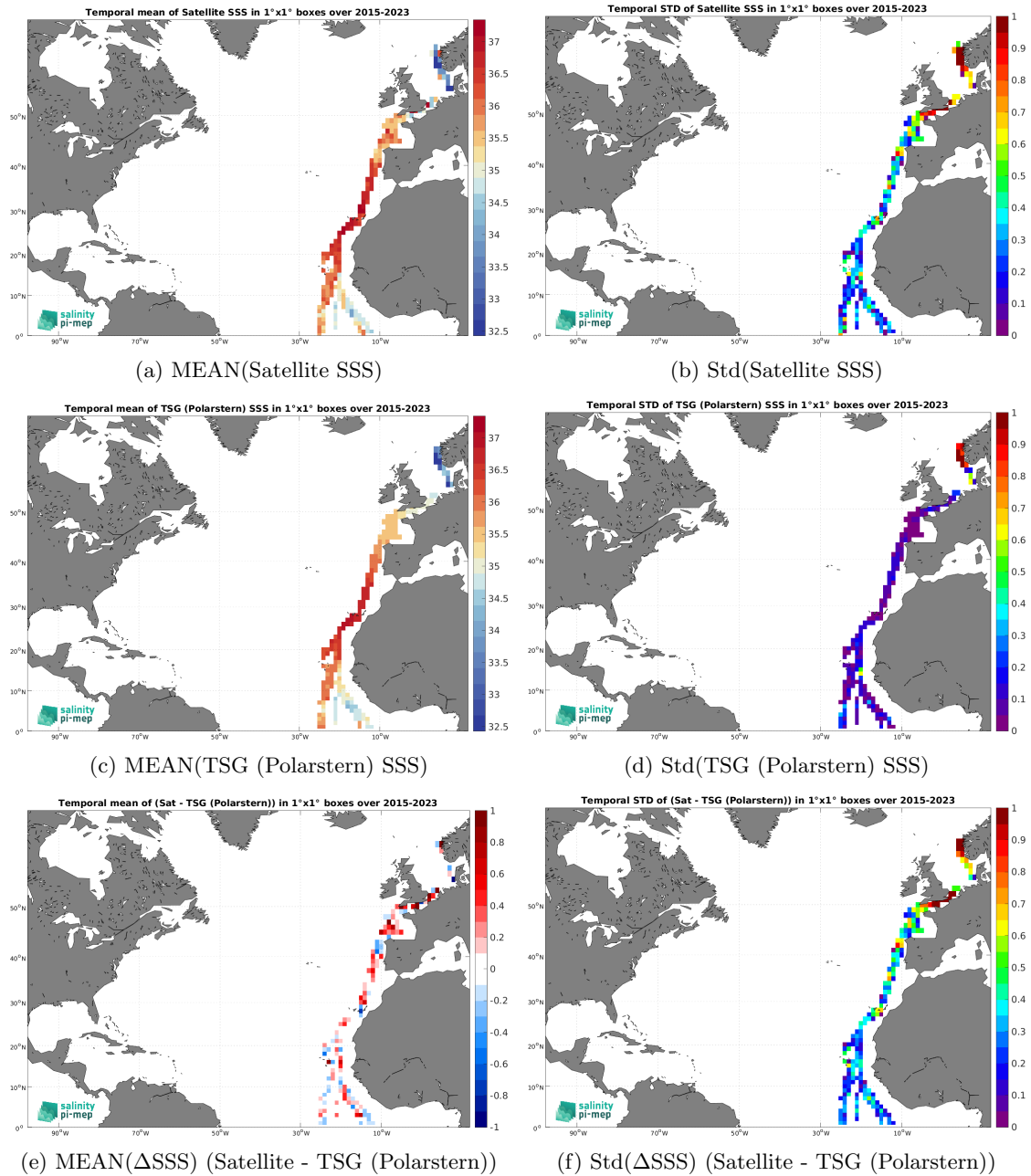
Figure 7: Temporal mean (left) and Std (right) of SSS from SMAP SSS L2 v6 (RSS) (top), TSG (Polarstern) (middle), and of \Delta SSS (Satellite - TSG (Polarstern)). Only match-up pairs are used to generate these maps.
